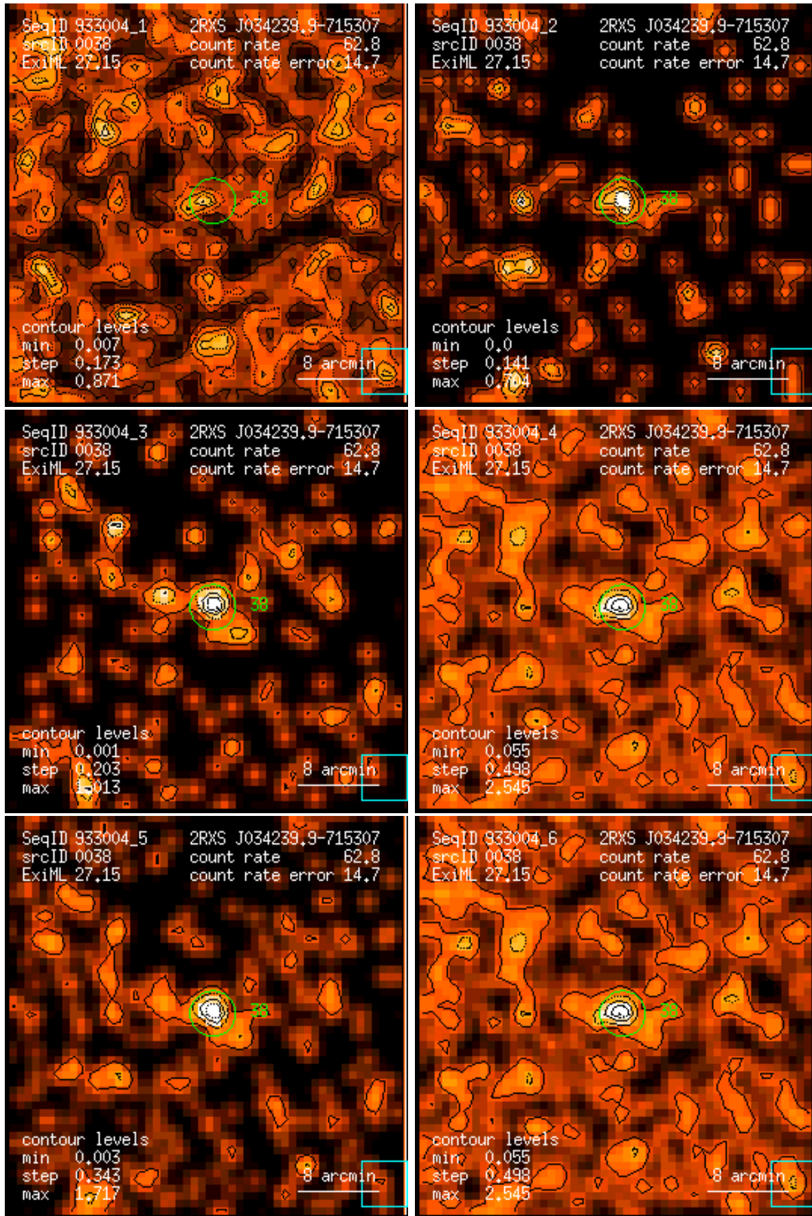
Figure 38: RASS 933004: detection 0038: band rate images, Gaussian filter: (1) PSPC channels 11 – 41, (2) 52 – 90, (3) 91 – 201, (4) 11 – 235, (5) 52 – 201, (6) 11 – 201. Broad band rates in counts/ks. Band rate contour levels in counts/ks/arcmin 2 .
