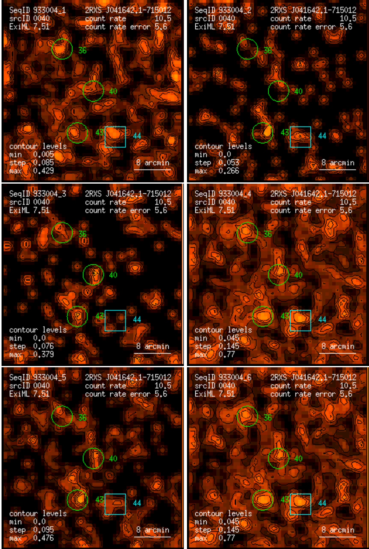
Figure 40: RASS 933004: detection 0040: band rate images, Gaussian filter: (1) PSPC channels 11 – 41, (2) 52 – 90, (3) 91 – 201, (4) 11 – 235, (5) 52 – 201, (6) 11 – 201. Broad band rates in counts/ks. Band rate contour levels in counts/ks/arcmin 2 .
