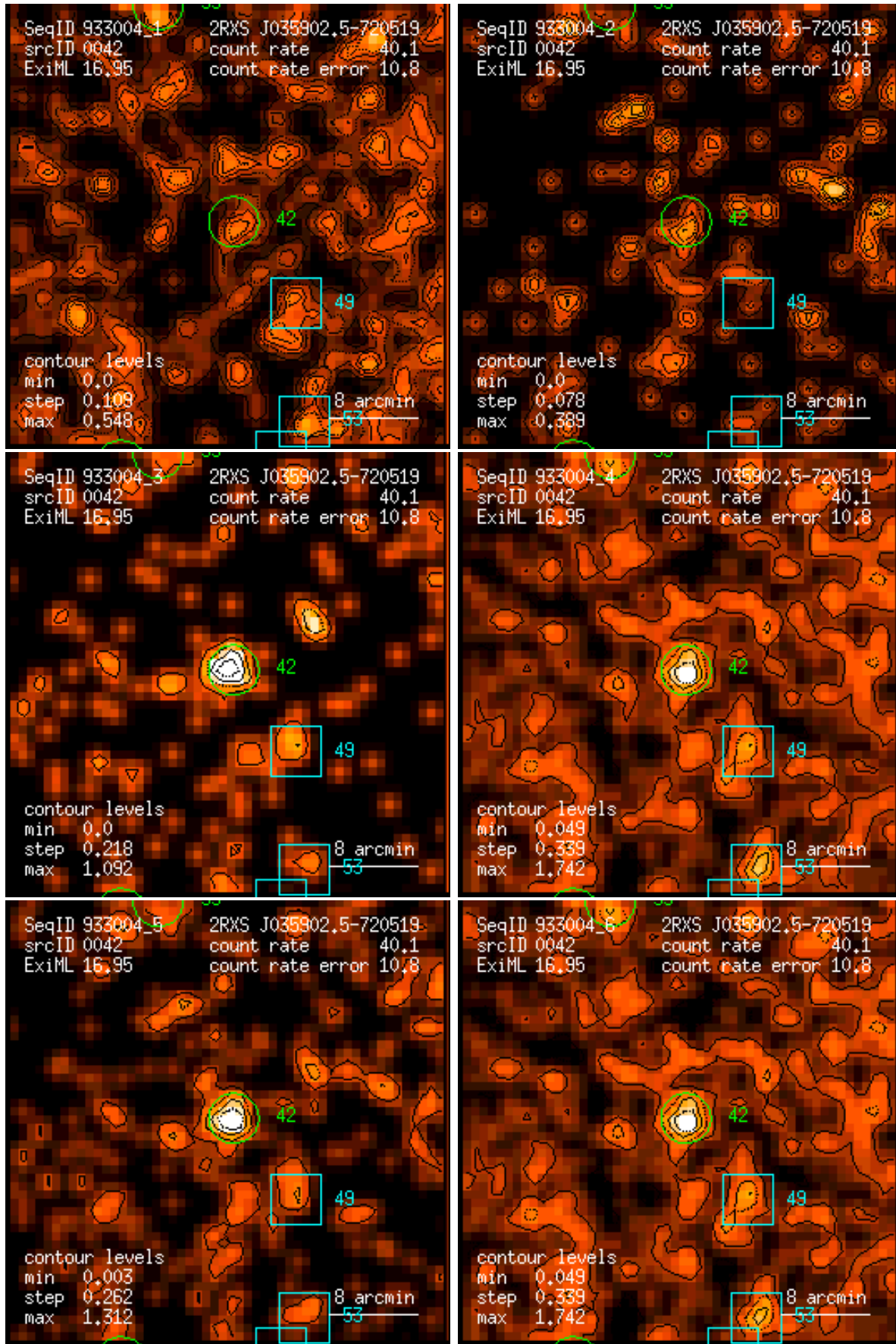
Figure 42: RASS 933004: detection 0042: band rate images, Gaussian filter: (1) PSPC channels 11 – 41, (2) 52 – 90, (3) 91 – 201, (4) 11 – 235, (5) 52 – 201, (6) 11 – 201. Broad band rates in counts/ks. Band rate contour levels in counts/ks/arcmin 2 .
