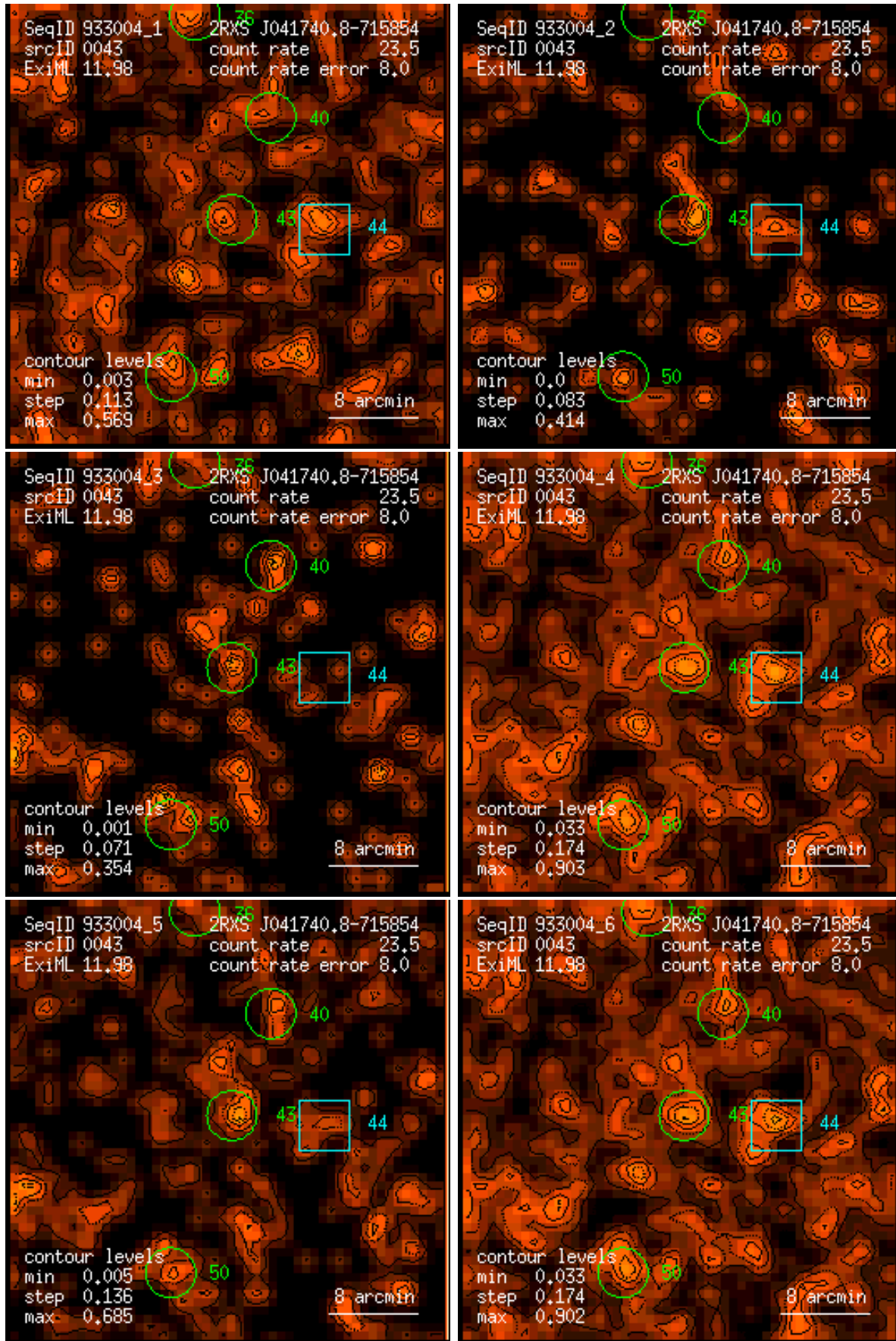
Figure 43: RASS 933004: detection 0043: band rate images, Gaussian filter: (1) PSPC channels 11 – 41, (2) 52 – 90, (3) 91 – 201, (4) 11 – 235, (5) 52 – 201, (6) 11 – 201. Broad band rates in counts/ks. Band rate contour levels in counts/ks/arcmin 2 .
