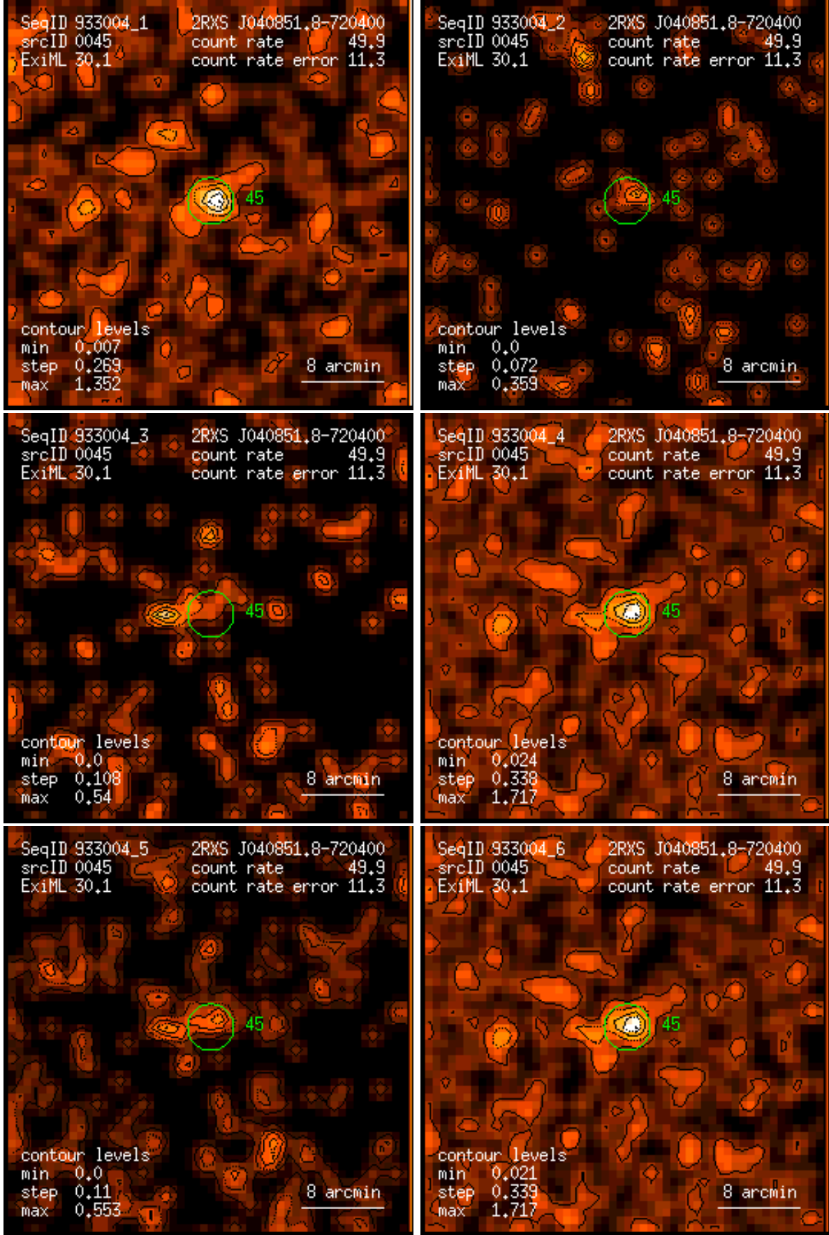
Figure 45: RASS 933004: detection 0045: band rate images, Gaussian filter: (1) PSPC channels 11 – 41, (2) 52 – 90, (3) 91 – 201, (4) 11 – 235, (5) 52 – 201, (6) 11 – 201. Broad band rates in counts/ks. Band rate contour levels in counts/ks/arcmin 2 .
