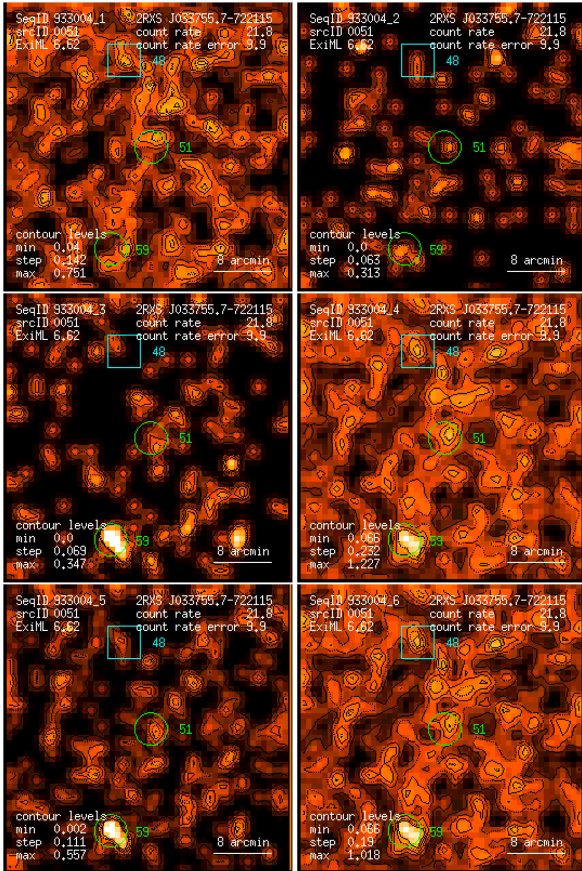
Figure 51: RASS 933004: detection 0051: band rate images, Gaussian filter: (1) PSPC channels 11 – 41, (2) 52 – 90, (3) 91 – 201, (4) 11 – 235, (5) 52 – 201, (6) 11 – 201. Broad band rates in counts/ks. Band rate contour levels in counts/ks/arcmin 2 .
