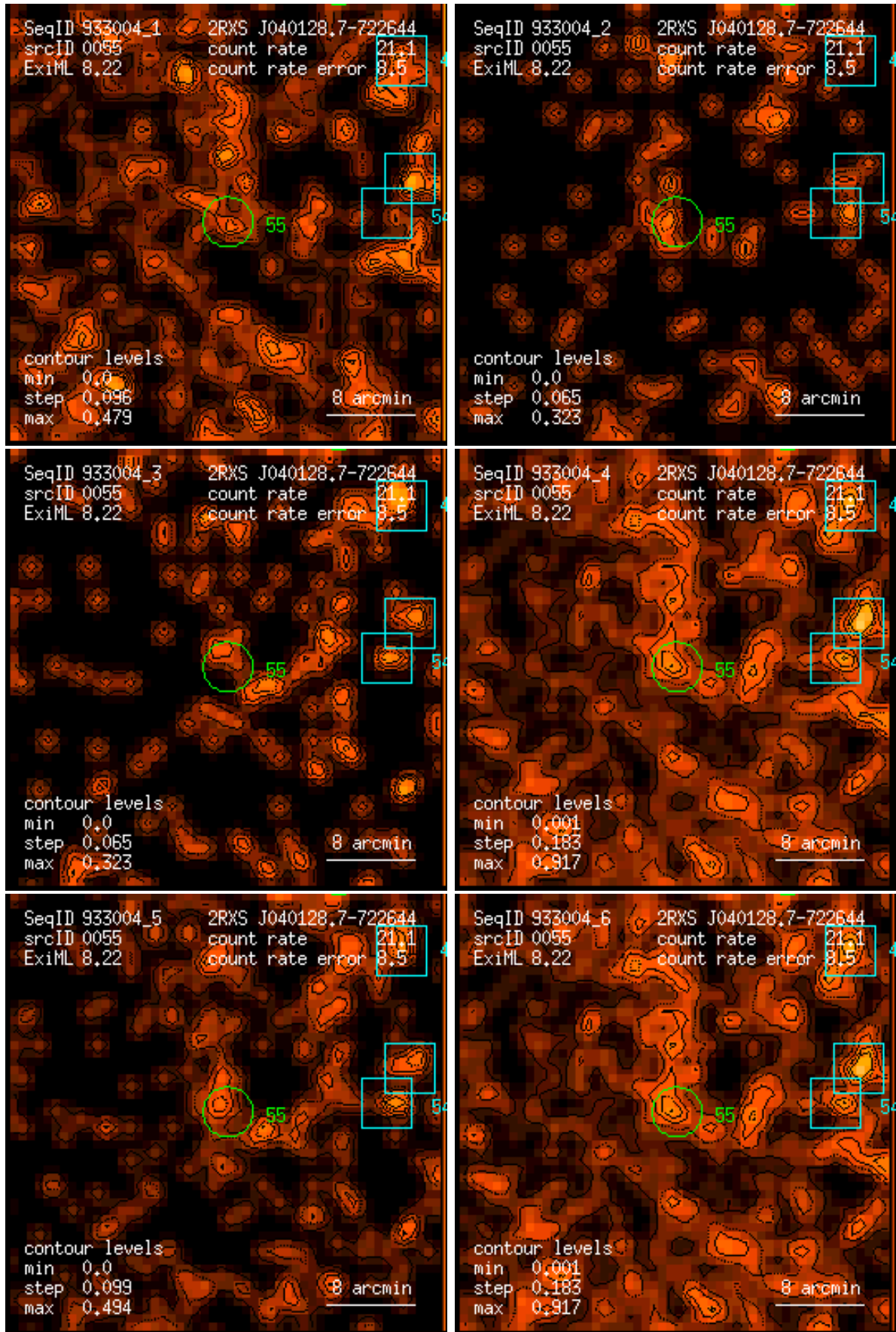
Figure 55: RASS 933004: detection 0055: band rate images, Gaussian filter: (1) PSPC channels 11 – 41, (2) 52 – 90, (3) 91 – 201, (4) 11 – 235, (5) 52 – 201, (6) 11 – 201. Broad band rates in counts/ks. Band rate contour levels in counts/ks/arcmin 2 .
