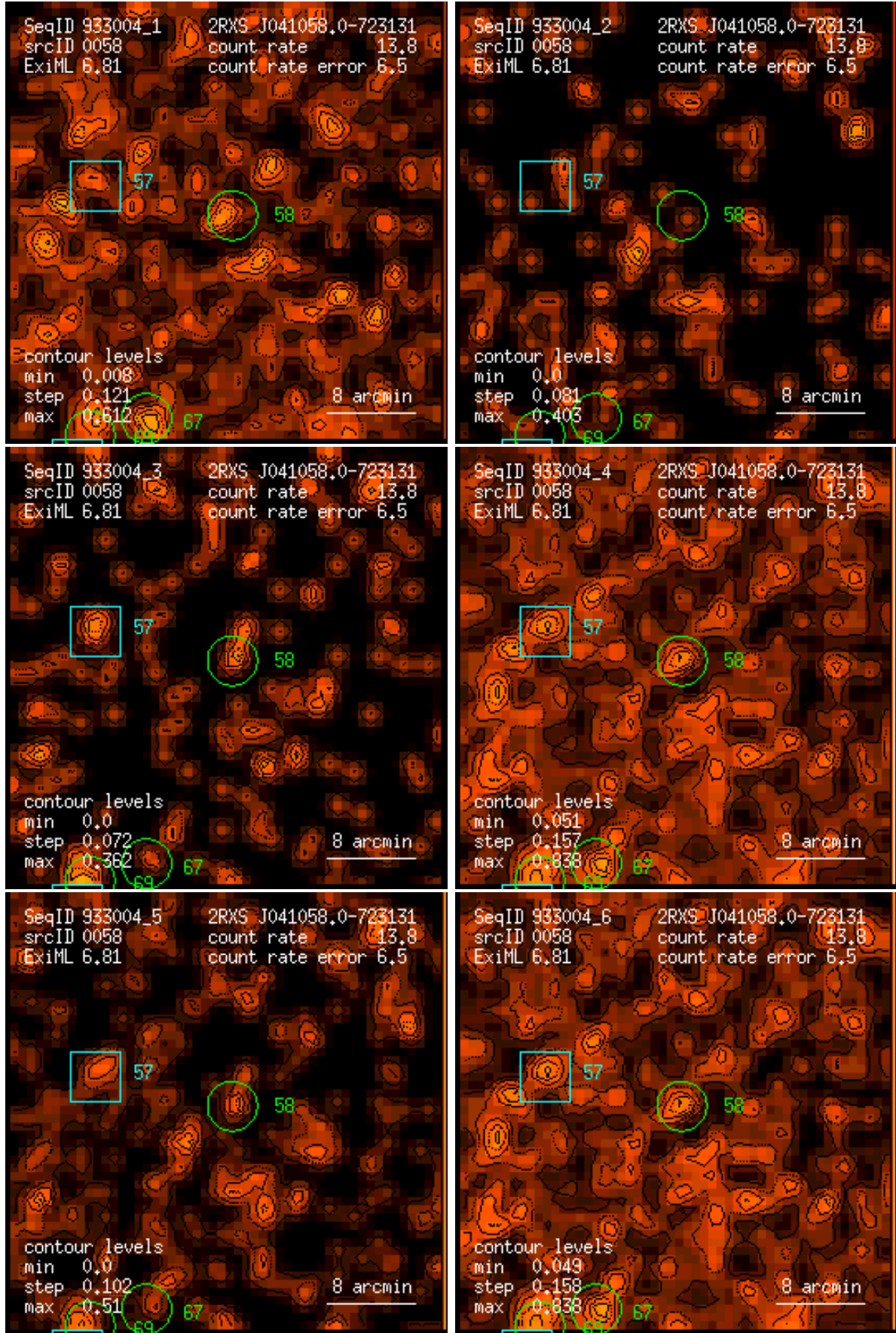
Figure 58: RASS 933004: detection 0058: band rate images, Gaussian filter: (1) PSPC channels 11 – 41, (2) 52 – 90, (3) 91 – 201, (4) 11 – 235, (5) 52 – 201, (6) 11 – 201. Broad band rates in counts/ks. Band rate contour levels in counts/ks/arcmin 2 .
