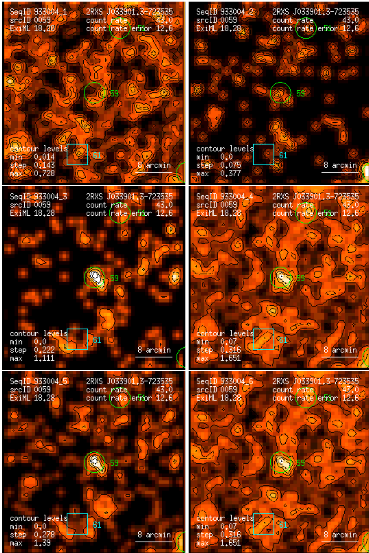
Figure 59: RASS 933004: detection 0059: band rate images, Gaussian filter: (1) PSPC channels 11 – 41, (2) 52 – 90, (3) 91 – 201, (4) 11 – 235, (5) 52 – 201, (6) 11 – 201. Broad band rates in counts/ks. Band rate contour levels in counts/ks/arcmin 2 .
