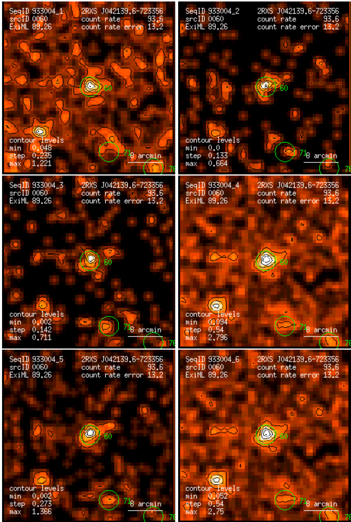
Figure 60: RASS 933004: detection 0060: band rate images, Gaussian filter: (1) PSPC channels 11 – 41, (2) 52 – 90, (3) 91 – 201, (4) 11 – 235, (5) 52 – 201, (6) 11 – 201. Broad band rates in counts/ks. Band rate contour levels in counts/ks/arcmin 2 .
