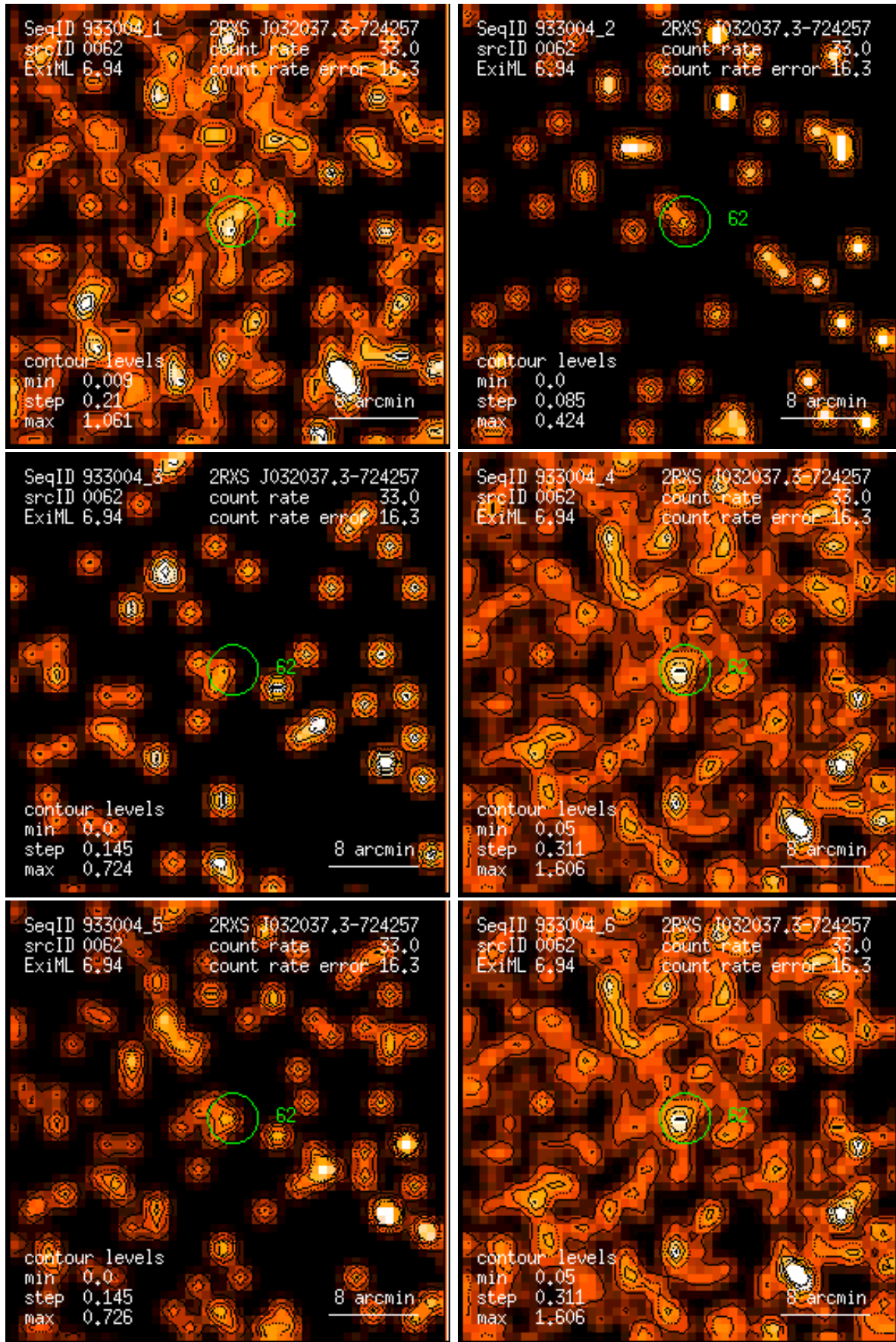
Figure 62: RASS 933004: detection 0062: band rate images, Gaussian filter: (1) PSPC channels 11 – 41, (2) 52 – 90, (3) 91 – 201, (4) 11 – 235, (5) 52 – 201, (6) 11 – 201. Broad band rates in counts/ks. Band rate contour levels in counts/ks/arcmin 2 .
