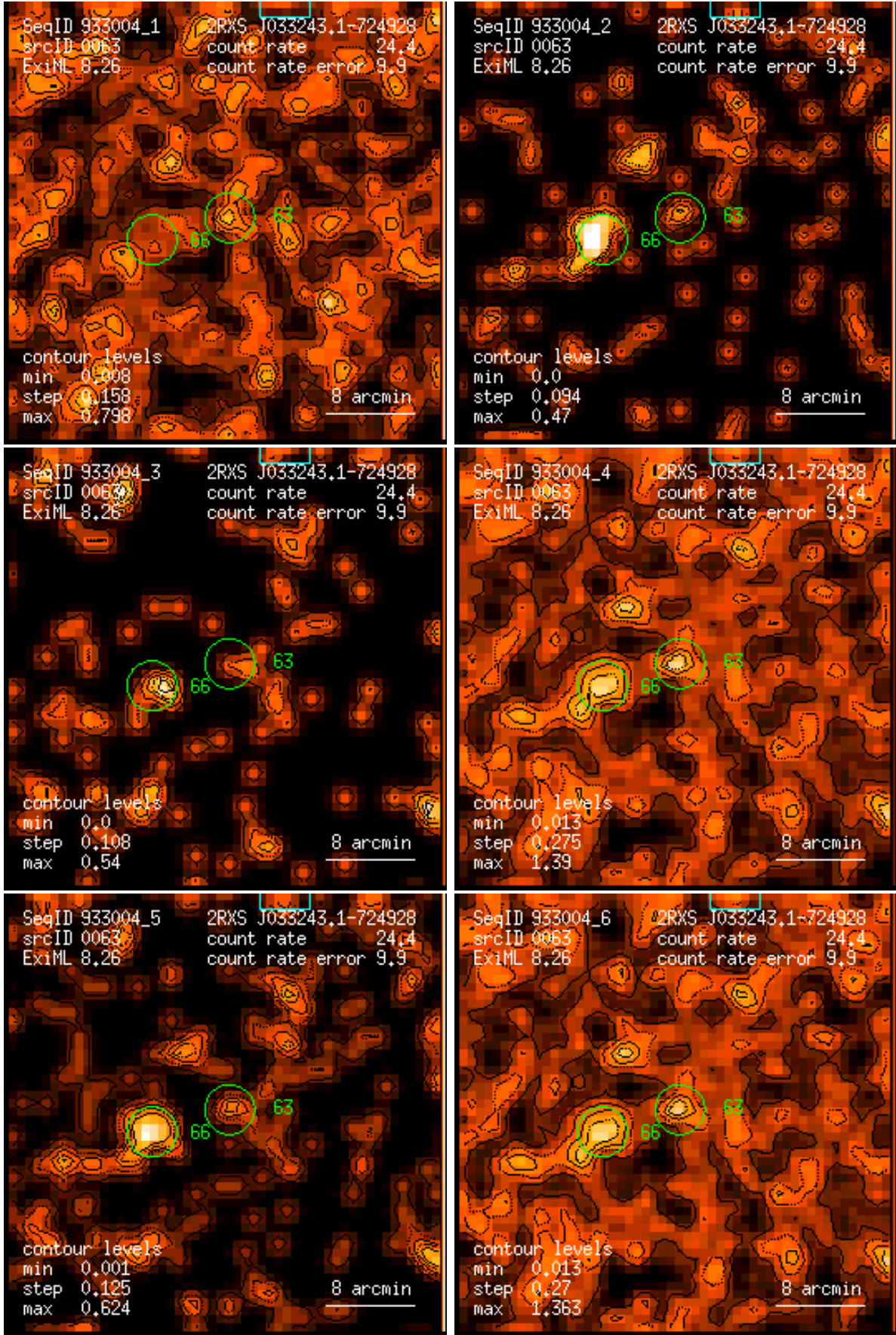
Figure 63: RASS 933004: detection 0063: band rate images, Gaussian filter: (1) PSPC channels 11 – 41, (2) 52 – 90, (3) 91 – 201, (4) 11 – 235, (5) 52 – 201, (6) 11 – 201. Broad band rates in counts/ks. Band rate contour levels in counts/ks/arcmin 2 .
