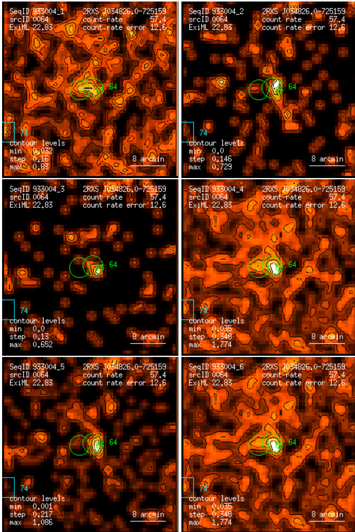
Figure 64: RASS 933004: detection 0064: band rate images, Gaussian filter: (1) PSPC channels 11 – 41, (2) 52 – 90, (3) 91 – 201, (4) 11 – 235, (5) 52 – 201, (6) 11 – 201. Broad band rates in counts/ks. Band rate contour levels in counts/ks/arcmin 2 .
