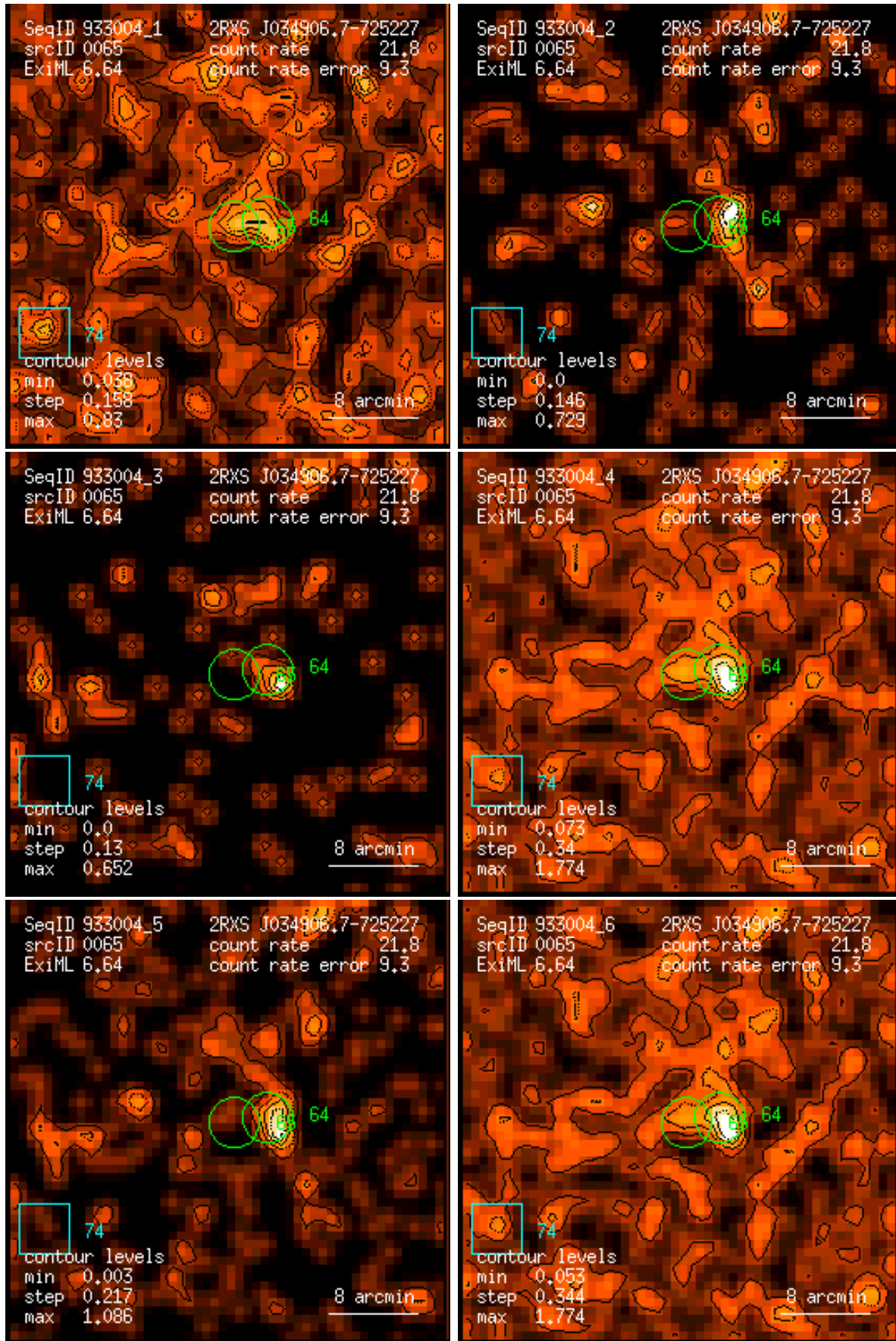
Figure 65: RASS 933004: detection 0065: band rate images, Gaussian filter: (1) PSPC channels 11 – 41, (2) 52 – 90, (3) 91 – 201, (4) 11 – 235, (5) 52 – 201, (6) 11 – 201. Broad band rates in counts/ks. Band rate contour levels in counts/ks/arcmin 2 .
