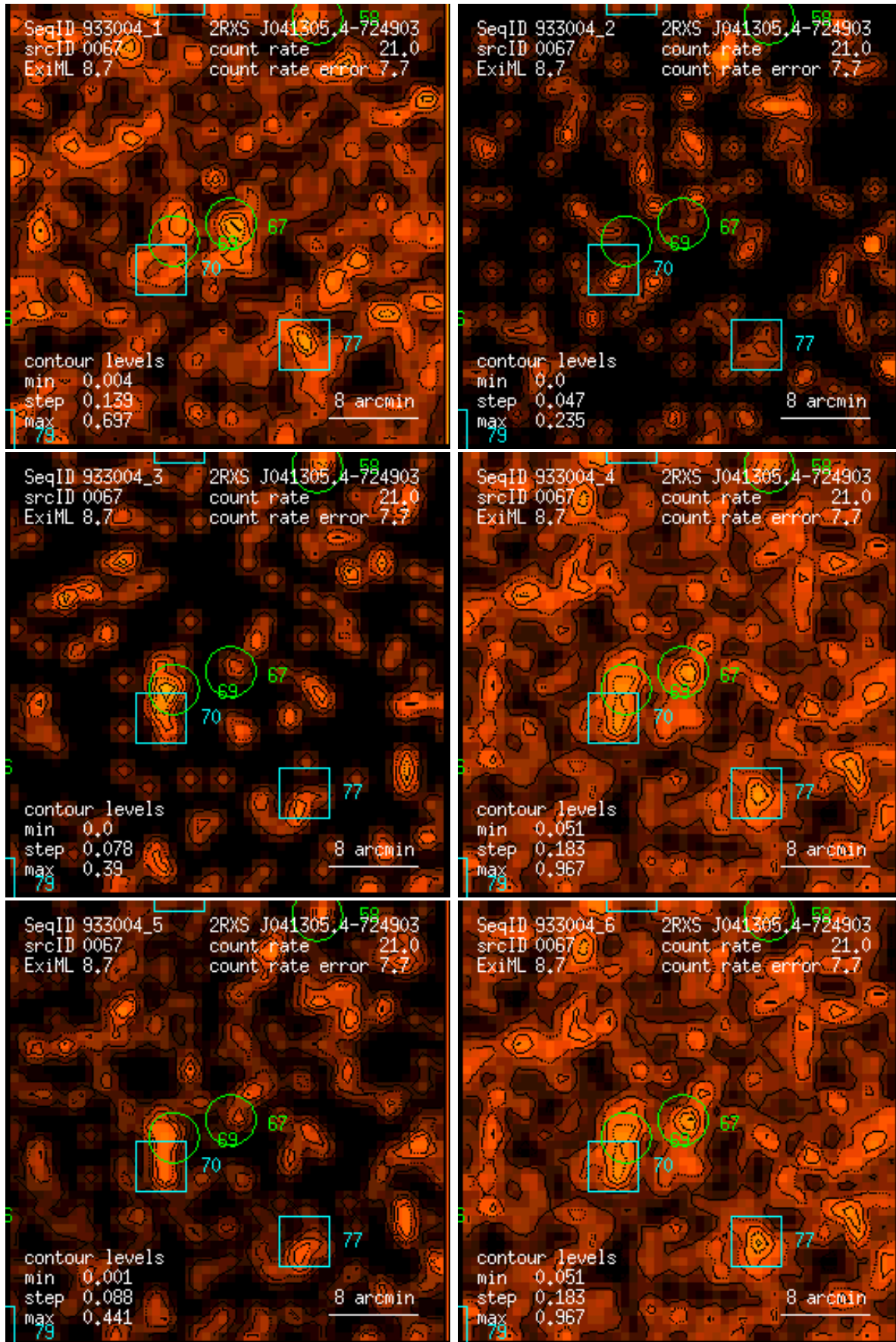
Figure 67: RASS 933004: detection 0067: band rate images, Gaussian filter: (1) PSPC channels 11 – 41, (2) 52 – 90, (3) 91 – 201, (4) 11 – 235, (5) 52 – 201, (6) 11 – 201. Broad band rates in counts/ks. Band rate contour levels in counts/ks/arcmin 2 .
