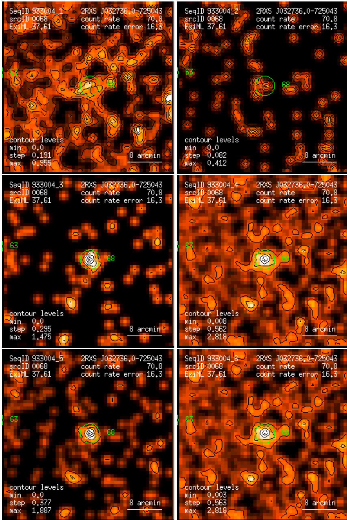
Figure 68: RASS 933004: detection 0068: band rate images, Gaussian filter: (1) PSPC channels 11 – 41, (2) 52 – 90, (3) 91 – 201, (4) 11 – 235, (5) 52 – 201, (6) 11 – 201. Broad band rates in counts/ks. Band rate contour levels in counts/ks/arcmin 2 .
