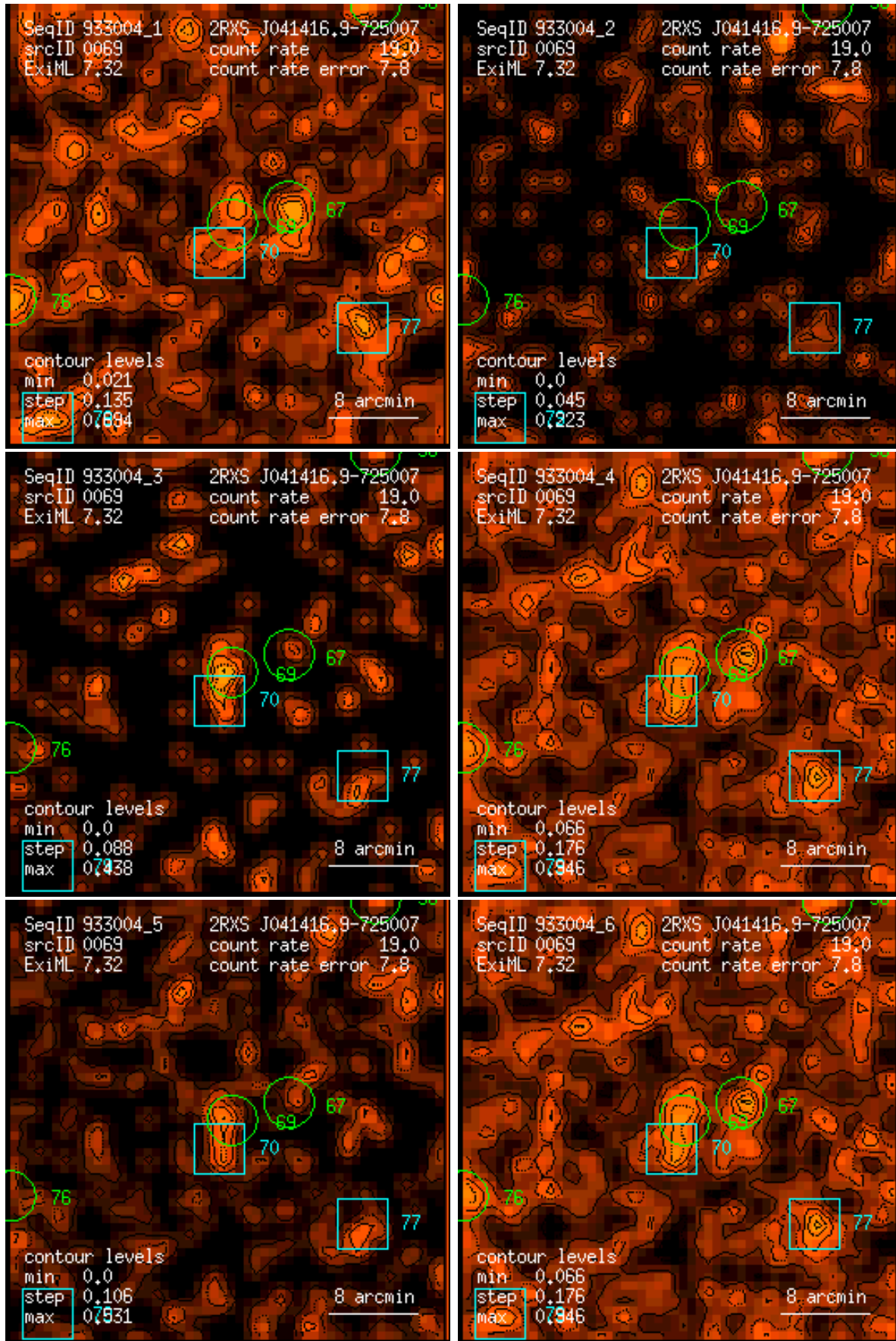
Figure 69: RASS 933004: detection 0069: band rate images, Gaussian filter: (1) PSPC channels 11 – 41, (2) 52 – 90, (3) 91 – 201, (4) 11 – 235, (5) 52 – 201, (6) 11 – 201. Broad band rates in counts/ks. Band rate contour levels in counts/ks/arcmin 2 .
