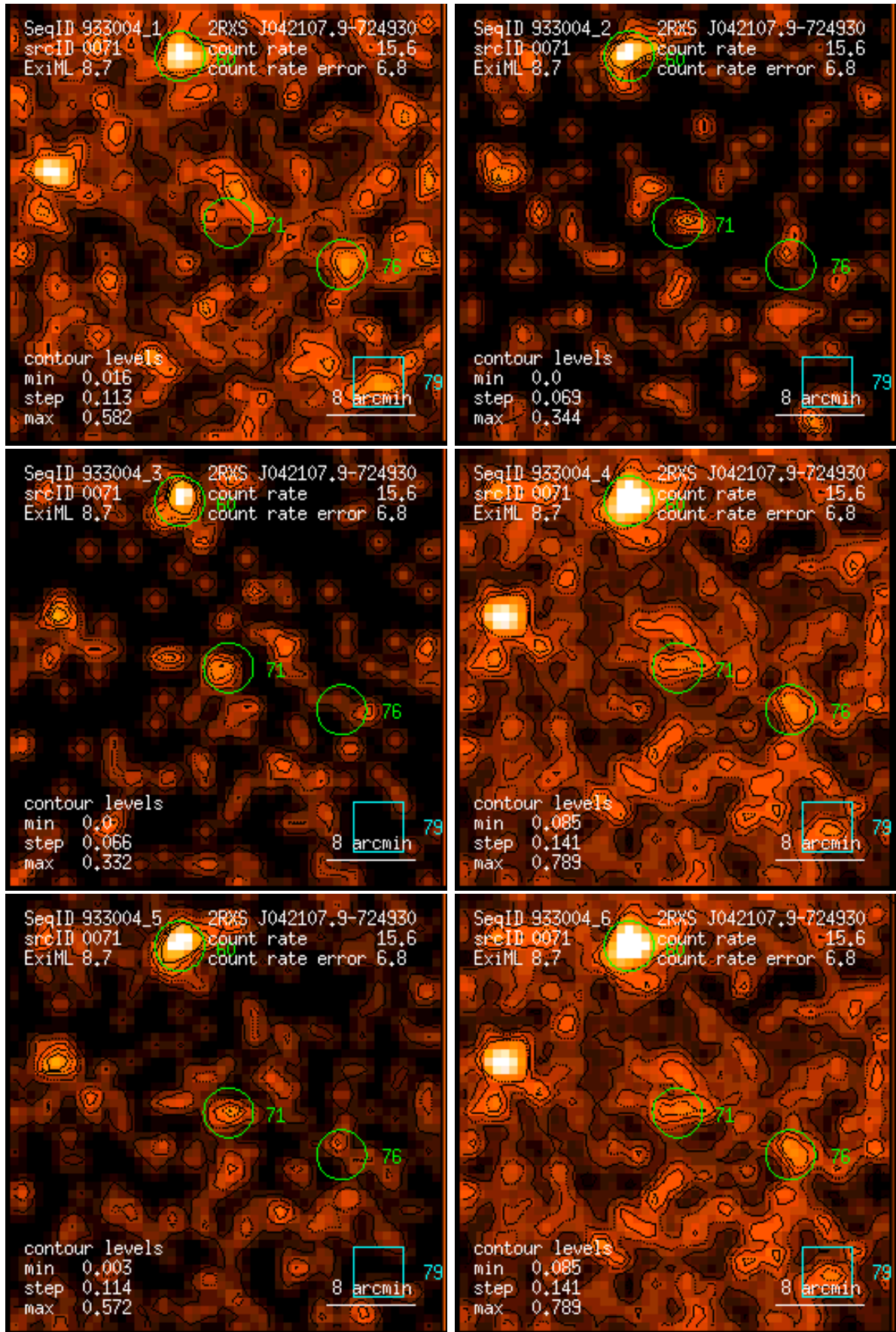
Figure 71: RASS 933004: detection 0071: band rate images, Gaussian filter: (1) PSPC channels 11 – 41, (2) 52 – 90, (3) 91 – 201, (4) 11 – 235, (5) 52 – 201, (6) 11 – 201. Broad band rates in counts/ks. Band rate contour levels in counts/ks/arcmin 2 .
