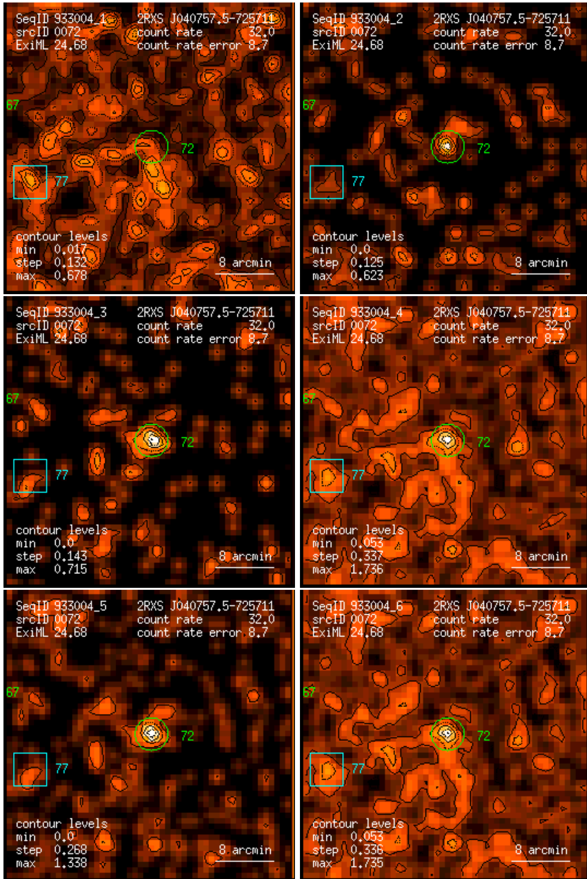
Figure 72: RASS 933004: detection 0072: band rate images, Gaussian filter: (1) PSPC channels 11 – 41, (2) 52 – 90, (3) 91 – 201, (4) 11 – 235, (5) 52 – 201, (6) 11 – 201. Broad band rates in counts/ks. Band rate contour levels in counts/ks/arcmin 2 .
