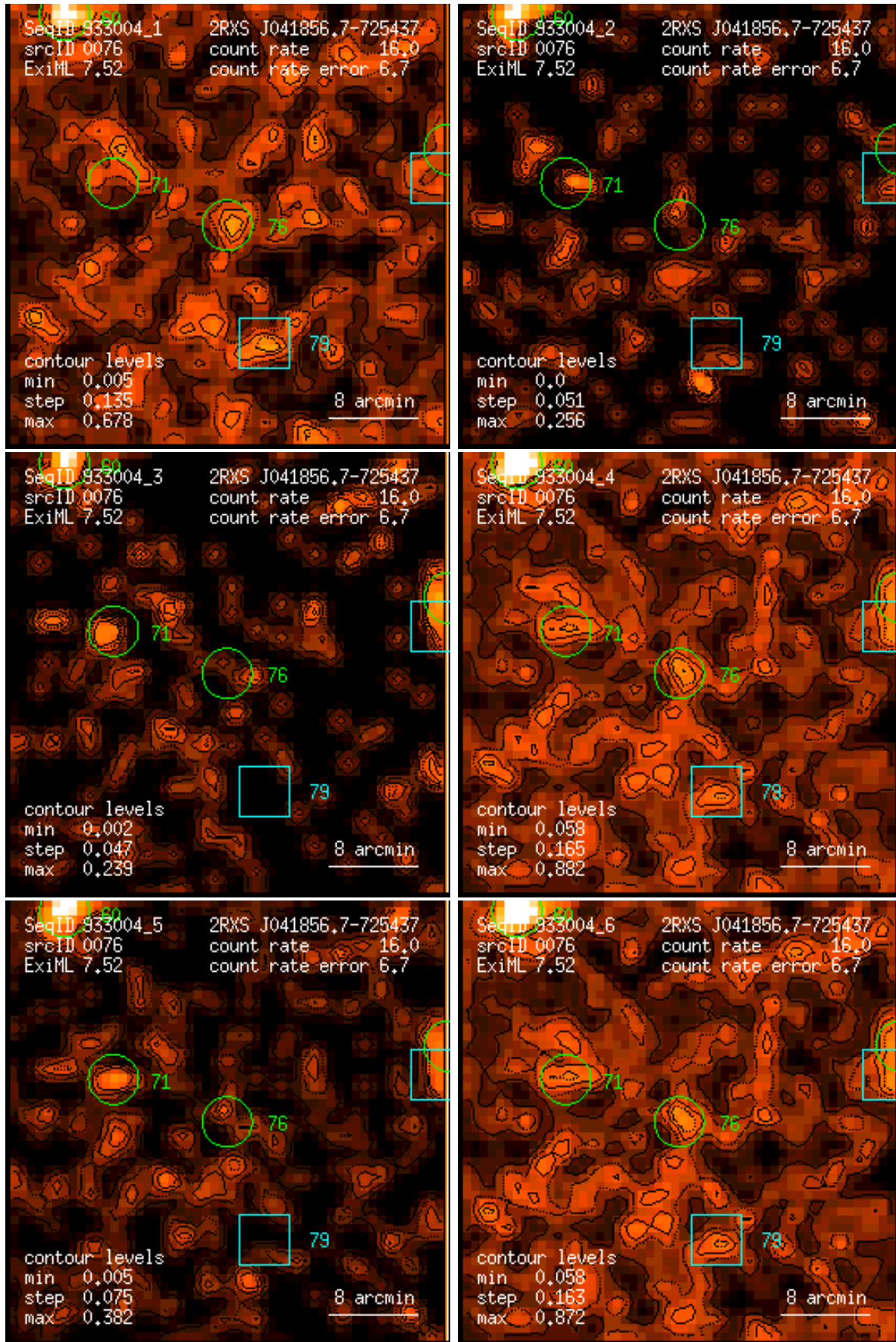
Figure 76: RASS 933004: detection 0076: band rate images, Gaussian filter: (1) PSPC channels 11 – 41, (2) 52 – 90, (3) 91 – 201, (4) 11 – 235, (5) 52 – 201, (6) 11 – 201. Broad band rates in counts/ks. Band rate contour levels in counts/ks/arcmin 2 .
