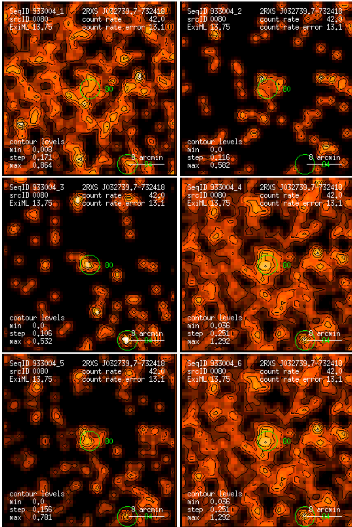
Figure 80: RASS 933004: detection 0080: band rate images, Gaussian filter: (1) PSPC channels 11 – 41, (2) 52 – 90, (3) 91 – 201, (4) 11 – 235, (5) 52 – 201, (6) 11 – 201. Broad band rates in counts/ks. Band rate contour levels in counts/ks/arcmin 2 .
