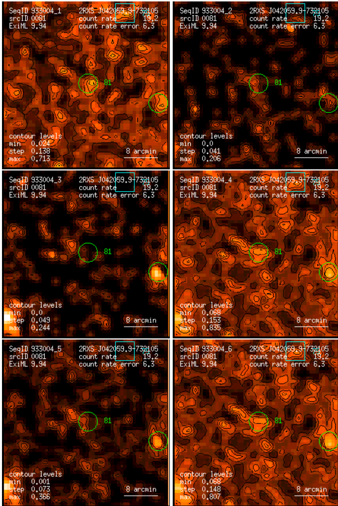
Figure 81: RASS 933004: detection 0081: band rate images, Gaussian filter: (1) PSPC channels 11 – 41, (2) 52 – 90, (3) 91 – 201, (4) 11 – 235, (5) 52 – 201, (6) 11 – 201. Broad band rates in counts/ks. Band rate contour levels in counts/ks/arcmin 2 .
