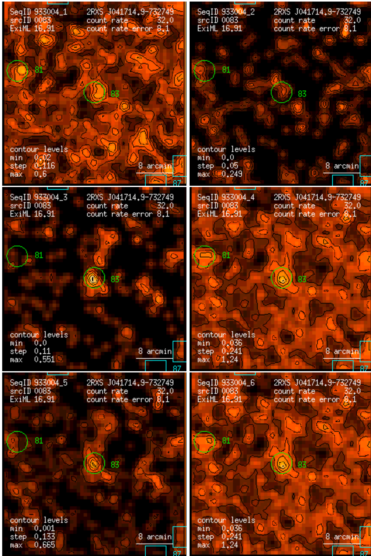
Figure 83: RASS 933004: detection 0083: band rate images, Gaussian filter: (1) PSPC channels 11 – 41, (2) 52 – 90, (3) 91 – 201, (4) 11 – 235, (5) 52 – 201, (6) 11 – 201. Broad band rates in counts/ks. Band rate contour levels in counts/ks/arcmin 2 .
