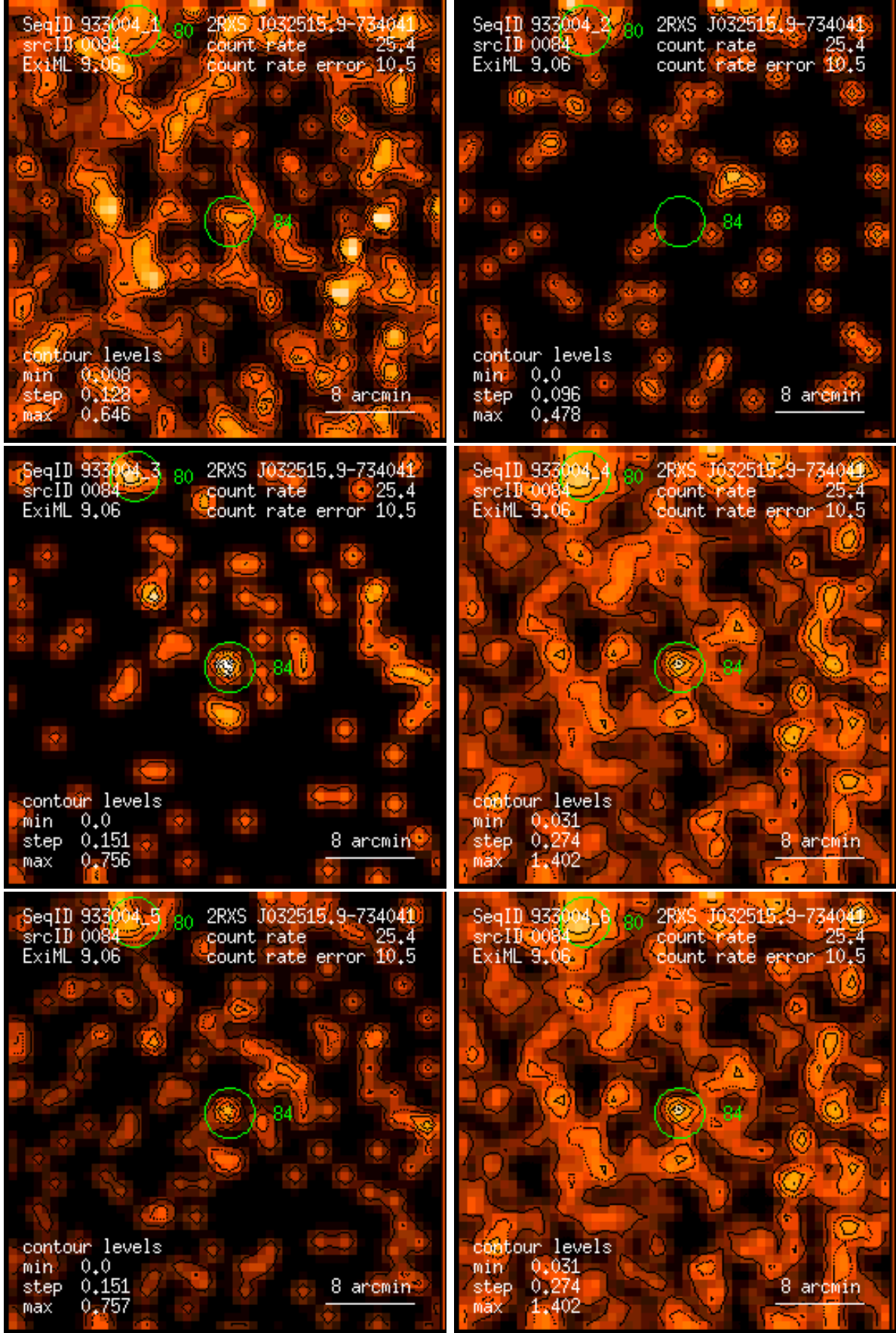
Figure 84: RASS 933004: detection 0084: band rate images, Gaussian filter: (1) PSPC channels 11 – 41, (2) 52 – 90, (3) 91 – 201, (4) 11 – 235, (5) 52 – 201, (6) 11 – 201. Broad band rates in counts/ks. Band rate contour levels in counts/ks/arcmin 2 .
