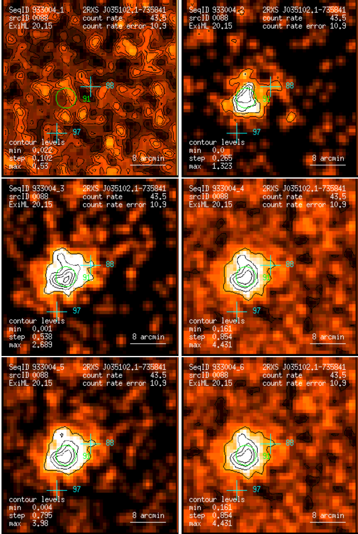
Figure 88: RASS 933004: detection 0088: band rate images, Gaussian filter: (1) PSPC channels 11 – 41, (2) 52 – 90, (3) 91 – 201, (4) 11 – 235, (5) 52 – 201, (6) 11 – 201. Broad band rates in counts/ks. Band rate contour levels in counts/ks/arcmin 2 .
