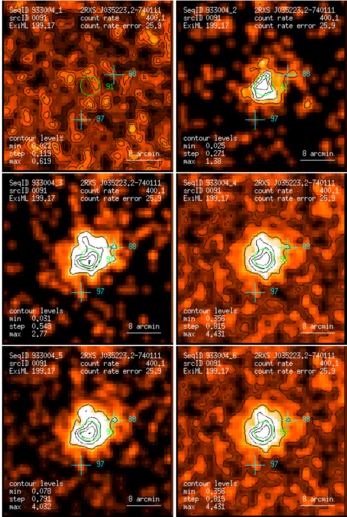
Figure 91: RASS 933004: detection 0091: band rate images, Gaussian filter: (1) PSPC channels 11 – 41, (2) 52 – 90, (3) 91 – 201, (4) 11 – 235, (5) 52 – 201, (6) 11 – 201. Broad band rates in counts/ks. Band rate contour levels in counts/ks/arcmin 2 .
