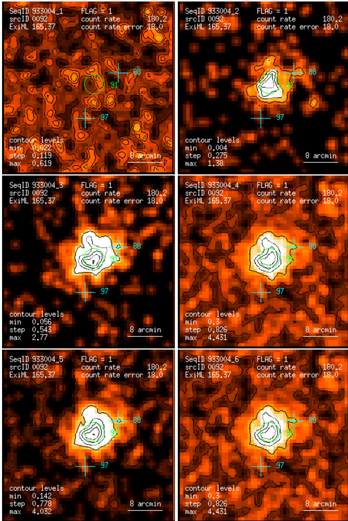
Figure 92: RASS 933004: detection 0092: band rate images, Gaussian filter: (1) PSPC channels 11 – 41, (2) 52 – 90, (3) 91 – 201, (4) 11 – 235, (5) 52 – 201, (6) 11 – 201. Broad band rates in counts/ks. Band rate contour levels in counts/ks/arcmin 2 .
