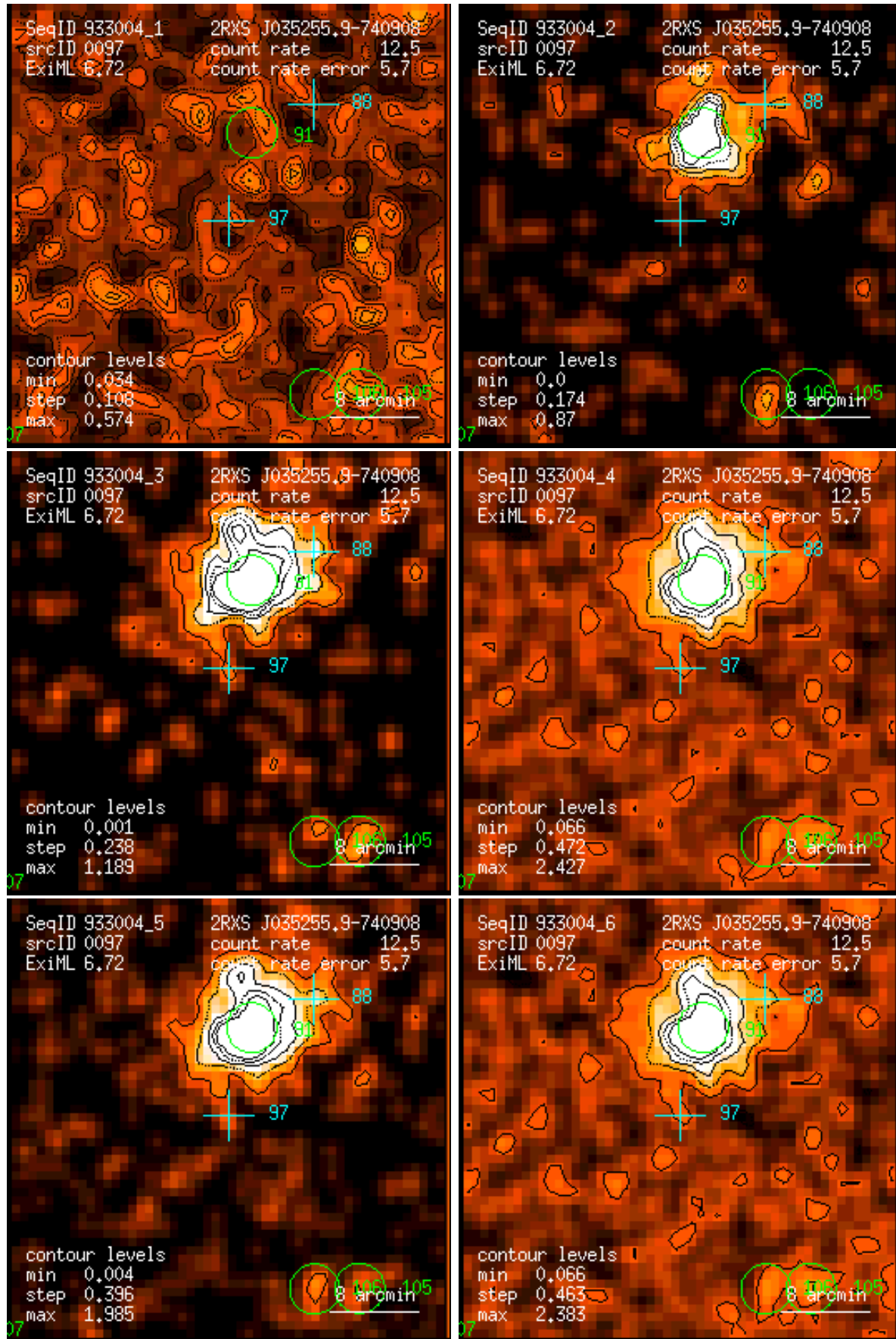
Figure 97: RASS 933004: detection 0097: band rate images, Gaussian filter: (1) PSPC channels 11 – 41, (2) 52 – 90, (3) 91 – 201, (4) 11 – 235, (5) 52 – 201, (6) 11 – 201. Broad band rates in counts/ks. Band rate contour levels in counts/ks/arcmin 2 .
