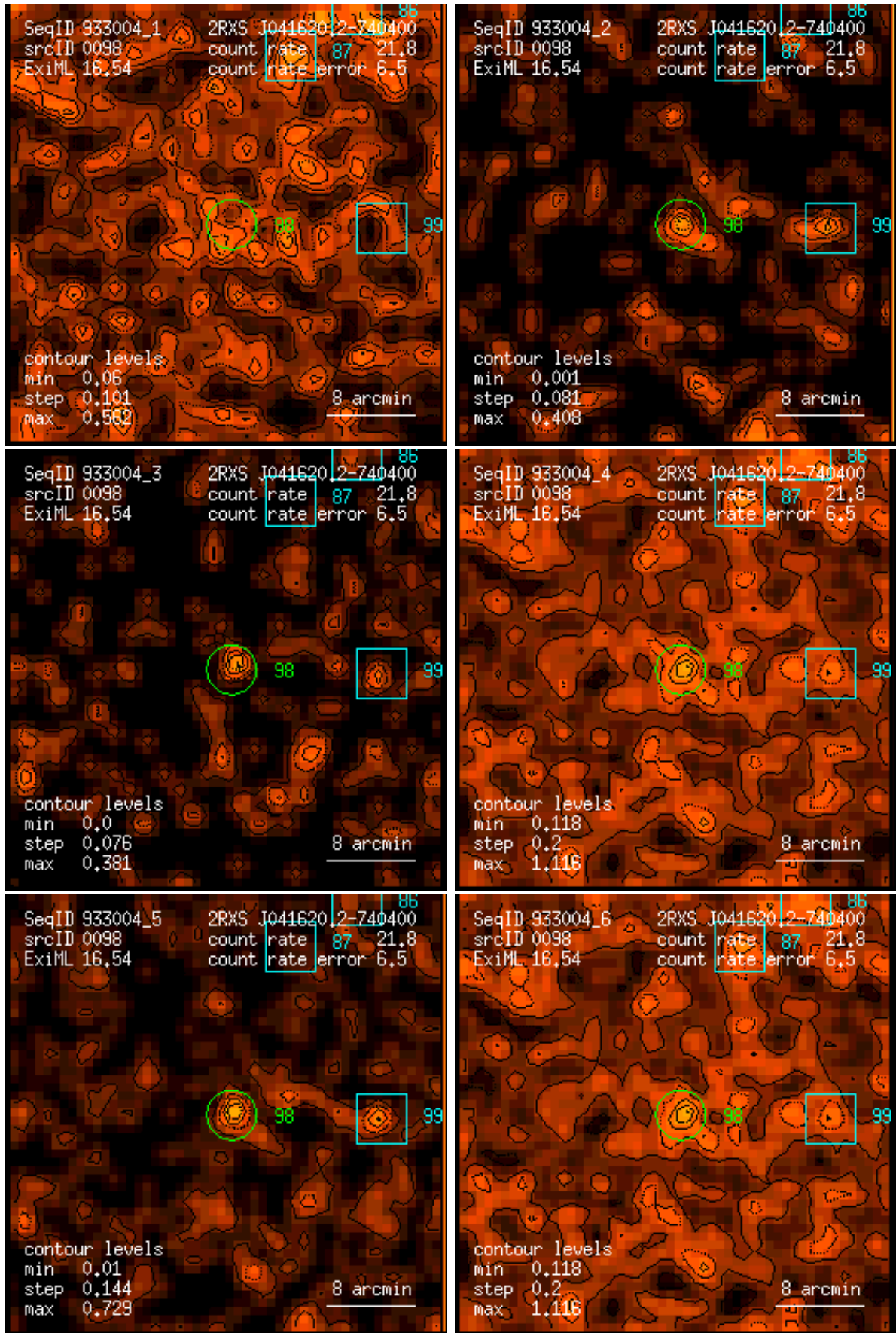
Figure 98: RASS 933004: detection 0098: band rate images, Gaussian filter: (1) PSPC channels 11 – 41, (2) 52 – 90, (3) 91 – 201, (4) 11 – 235, (5) 52 – 201, (6) 11 – 201. Broad band rates in counts/ks. Band rate contour levels in counts/ks/arcmin 2 .
