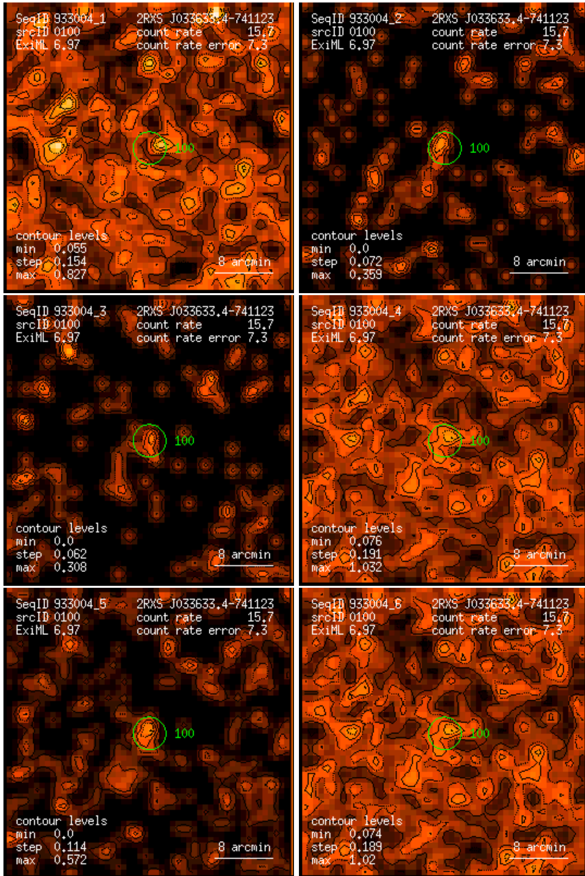
Figure 100: RASS 933004: detection 0100: band rate images, Gaussian filter: (1) PSPC channels 11 – 41, (2) 52 – 90, (3) 91 – 201, (4) 11 – 235, (5) 52 – 201, (6) 11 – 201. Broad band rates in counts/ks. Band rate contour levels in counts/ks/arcmin 2 .
