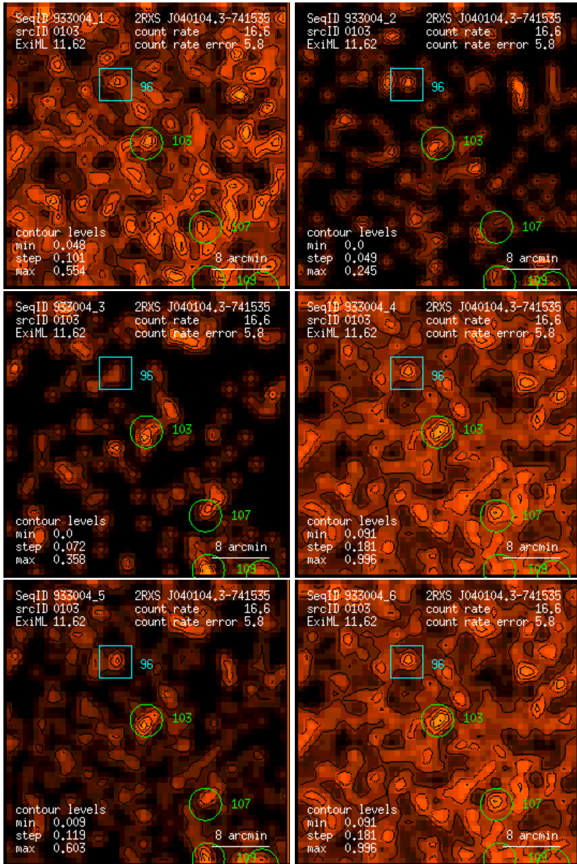
Figure 103: RASS 933004: detection 0103: band rate images, Gaussian filter: (1) PSPC channels 11 – 41, (2) 52 – 90, (3) 91 – 201, (4) 11 – 235, (5) 52 – 201, (6) 11 – 201. Broad band rates in counts/ks. Band rate contour levels in counts/ks/arcmin 2 .
