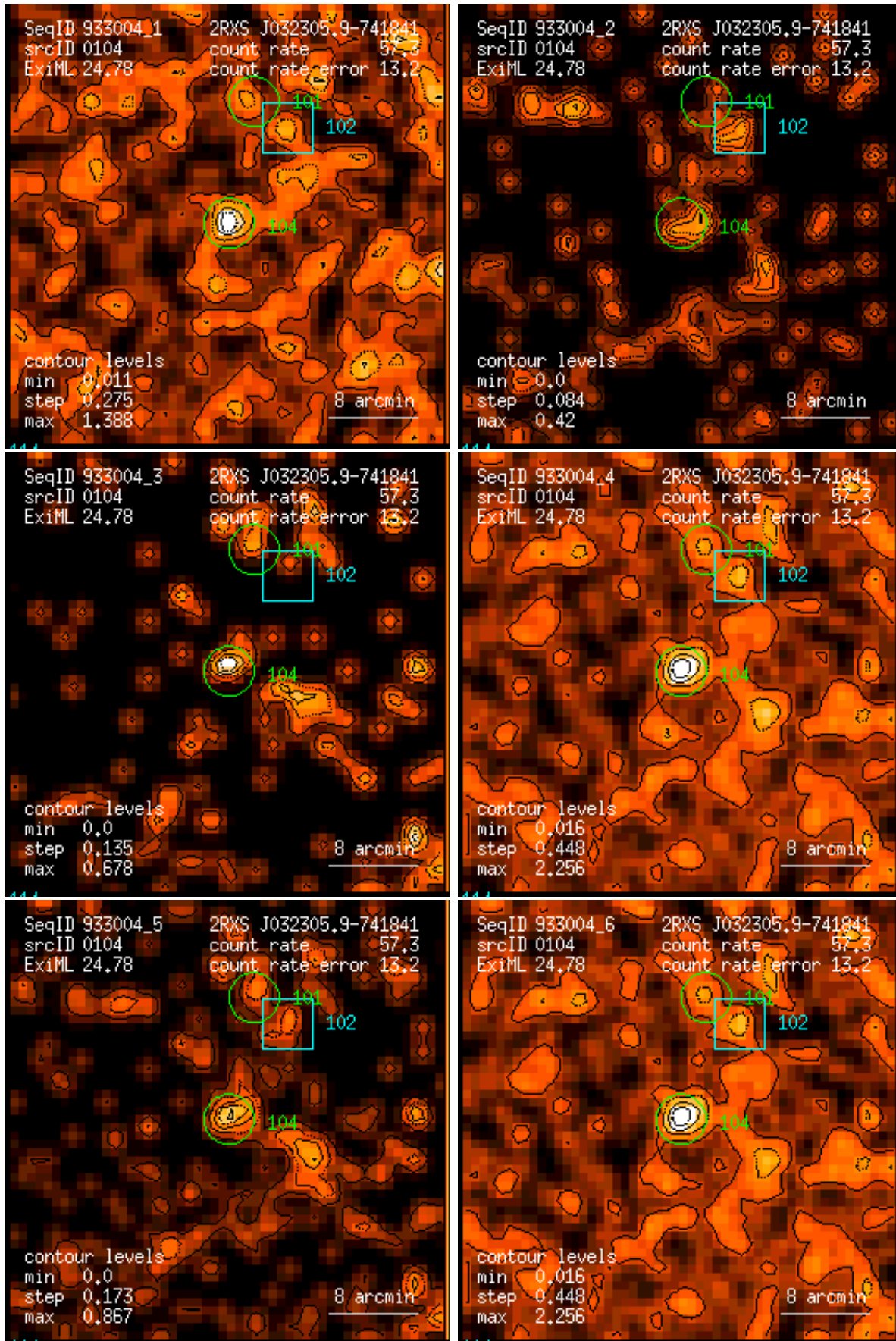
Figure 104: RASS 933004: detection 0104: band rate images, Gaussian filter: (1) PSPC channels 11 – 41, (2) 52 – 90, (3) 91 – 201, (4) 11 – 235, (5) 52 – 201, (6) 11 – 201. Broad band rates in counts/ks. Band rate contour levels in counts/ks/arcmin 2 .
