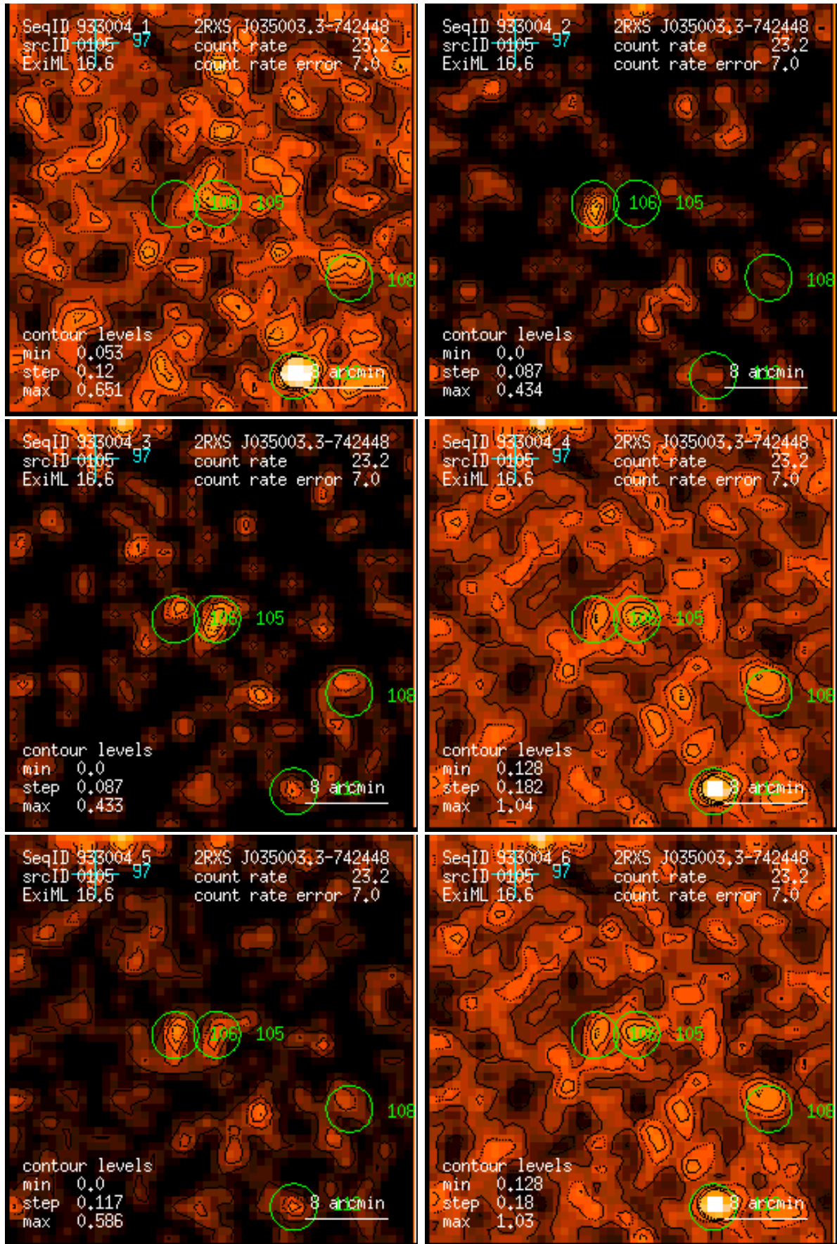
Figure 105: RASS 933004: detection 0105: band rate images, Gaussian filter: (1) PSPC channels 11 – 41, (2) 52 – 90, (3) 91 – 201, (4) 11 – 235, (5) 52 – 201, (6) 11 – 201. Broad band rates in counts/ks. Band rate contour levels in counts/ks/arcmin 2 .
