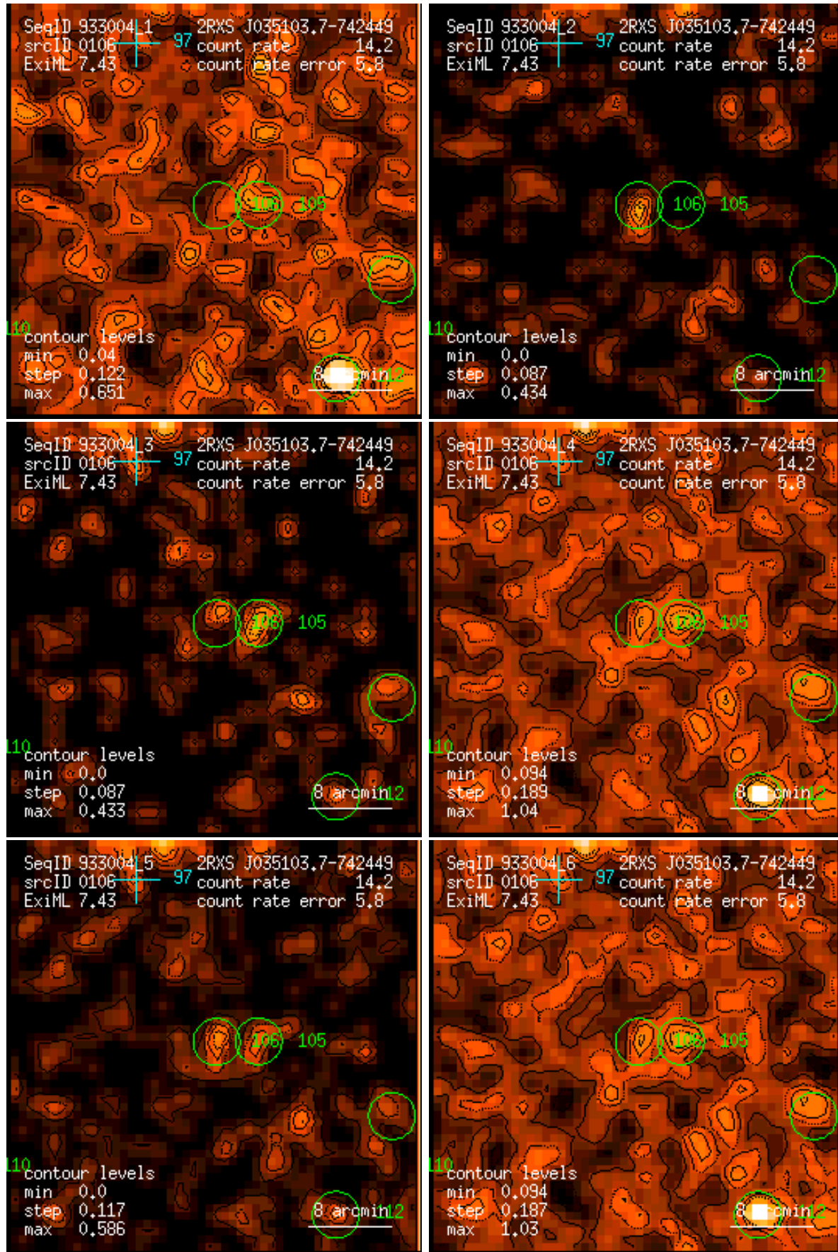
Figure 106: RASS 933004: detection 0106: band rate images, Gaussian filter: (1) PSPC channels 11 – 41, (2) 52 – 90, (3) 91 – 201, (4) 11 – 235, (5) 52 – 201, (6) 11 – 201. Broad band rates in counts/ks. Band rate contour levels in counts/ks/arcmin 2 .
