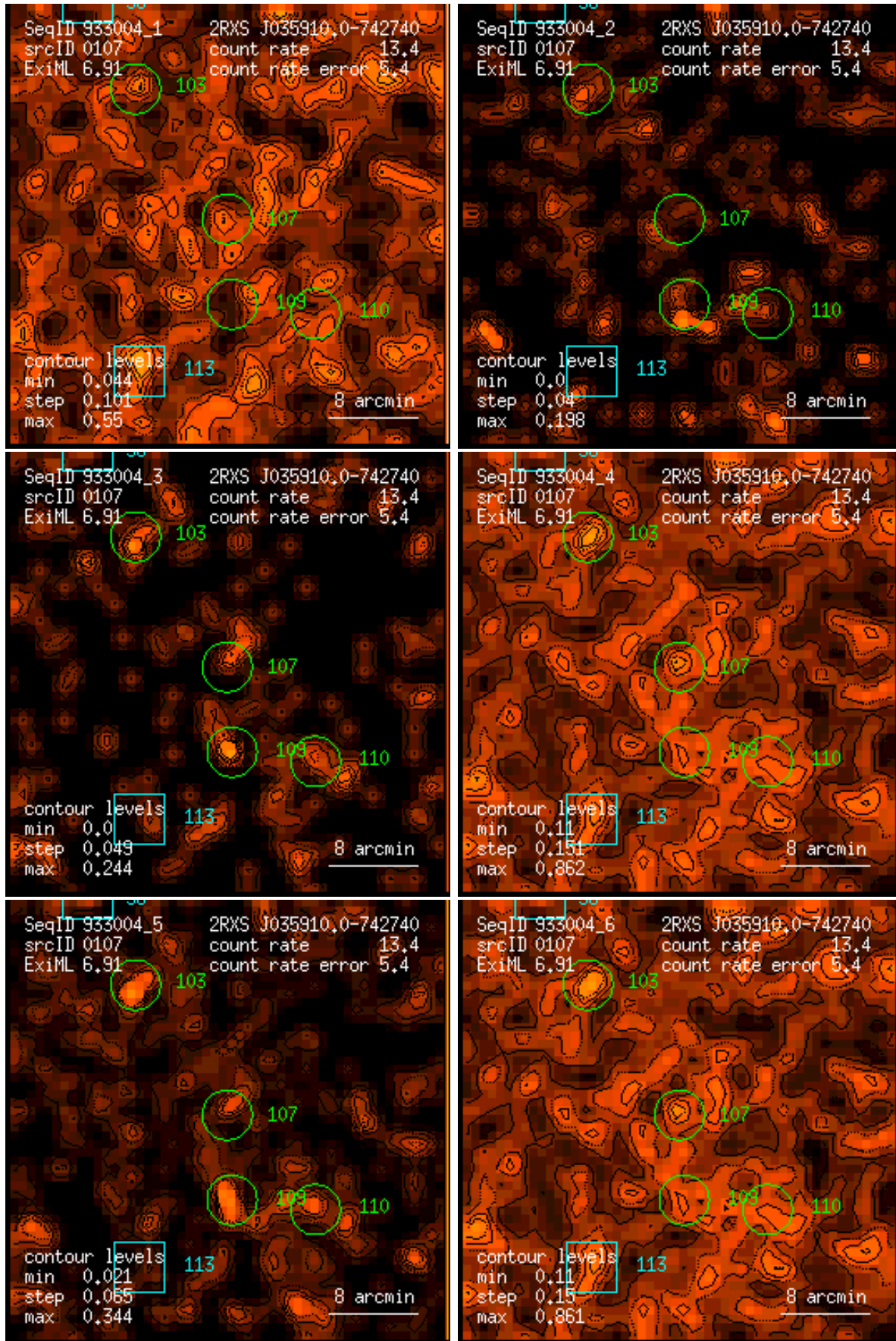
Figure 107: RASS 933004: detection 0107: band rate images, Gaussian filter: (1) PSPC channels 11 – 41, (2) 52 – 90, (3) 91 – 201, (4) 11 – 235, (5) 52 – 201, (6) 11 – 201. Broad band rates in counts/ks. Band rate contour levels in counts/ks/arcmin 2 .
