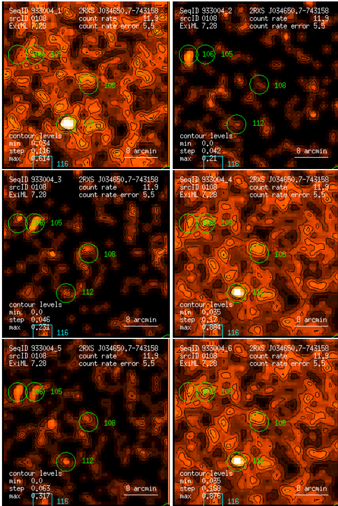
Figure 108: RASS 933004: detection 0108: band rate images, Gaussian filter: (1) PSPC channels 11 – 41, (2) 52 – 90, (3) 91 – 201, (4) 11 – 235, (5) 52 – 201, (6) 11 – 201. Broad band rates in counts/ks. Band rate contour levels in counts/ks/arcmin 2 .
