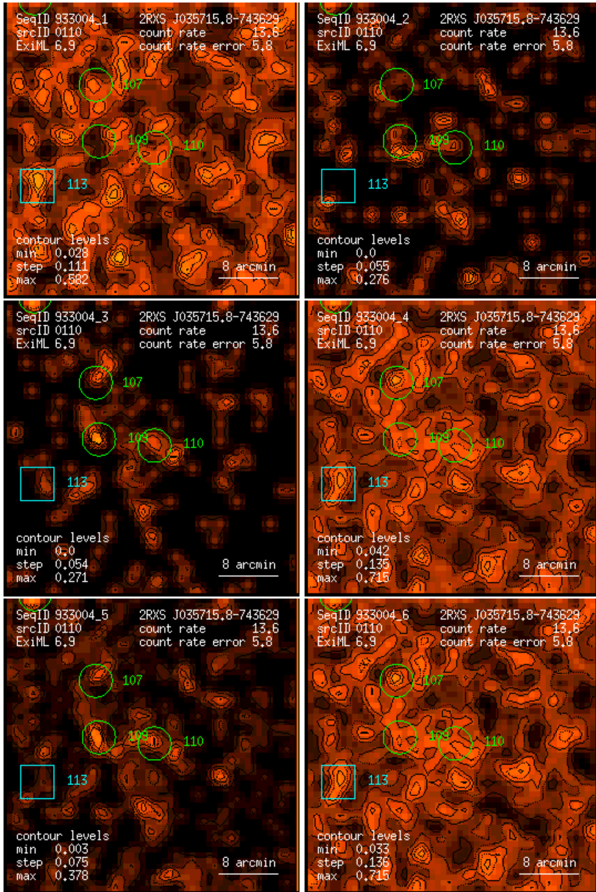
Figure 110: RASS 933004: detection 0110: band rate images, Gaussian filter: (1) PSPC channels 11 – 41, (2) 52 – 90, (3) 91 – 201, (4) 11 – 235, (5) 52 – 201, (6) 11 – 201. Broad band rates in counts/ks. Band rate contour levels in counts/ks/arcmin 2 .
