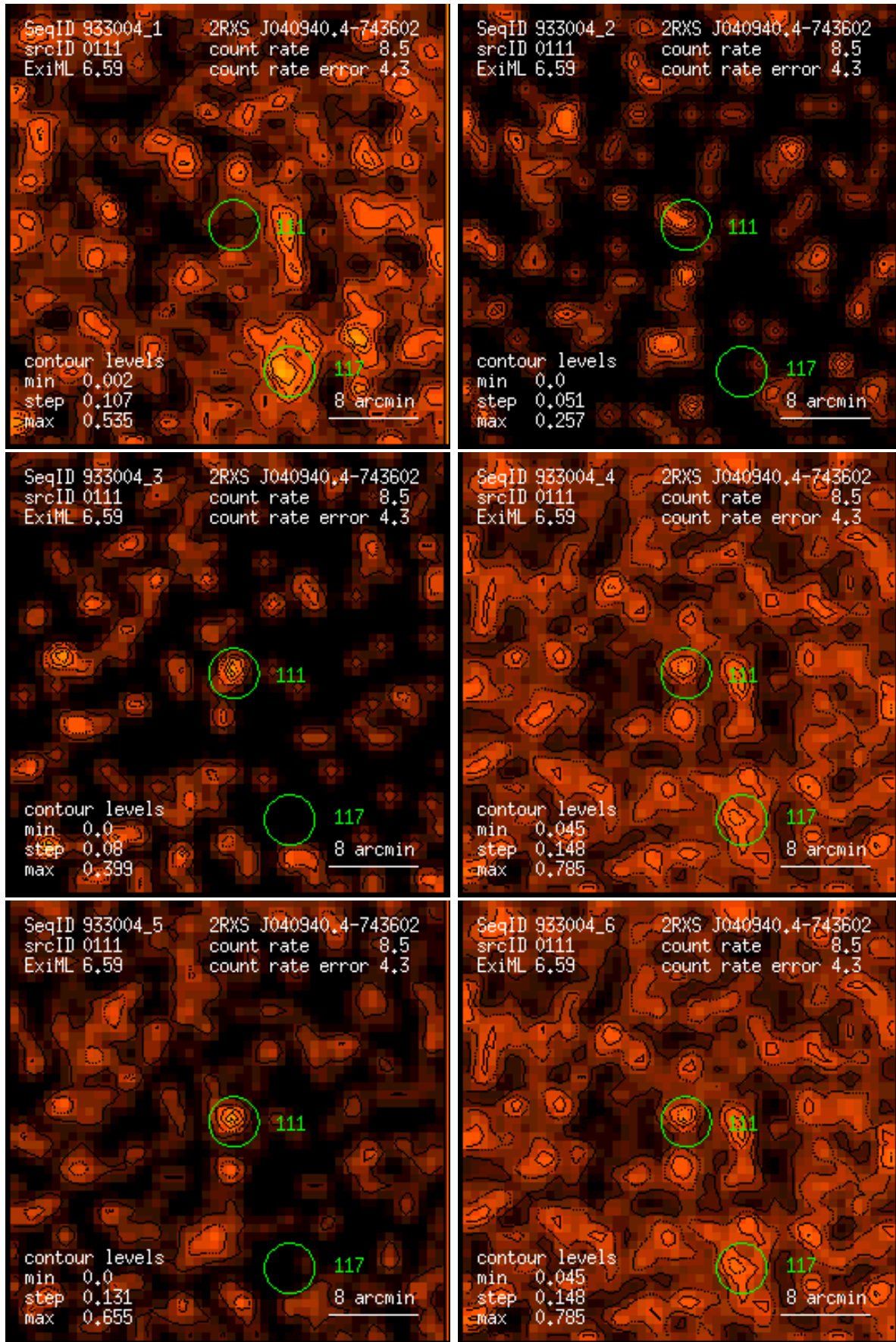
Figure 111: RASS 933004: detection 0111: band rate images, Gaussian filter: (1) PSPC channels 11 – 41, (2) 52 – 90, (3) 91 – 201, (4) 11 – 235, (5) 52 – 201, (6) 11 – 201. Broad band rates in counts/ks. Band rate contour levels in counts/ks/arcmin 2 .
