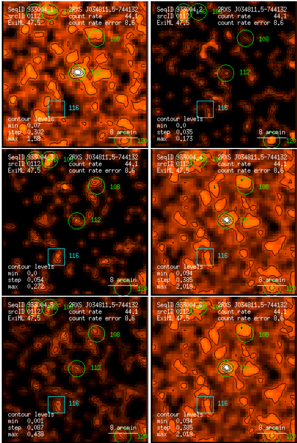
Figure 112: RASS 933004: detection 0112: band rate images, Gaussian filter: (1) PSPC channels 11 – 41, (2) 52 – 90, (3) 91 – 201, (4) 11 – 235, (5) 52 – 201, (6) 11 – 201. Broad band rates in counts/ks. Band rate contour levels in counts/ks/arcmin 2 .
