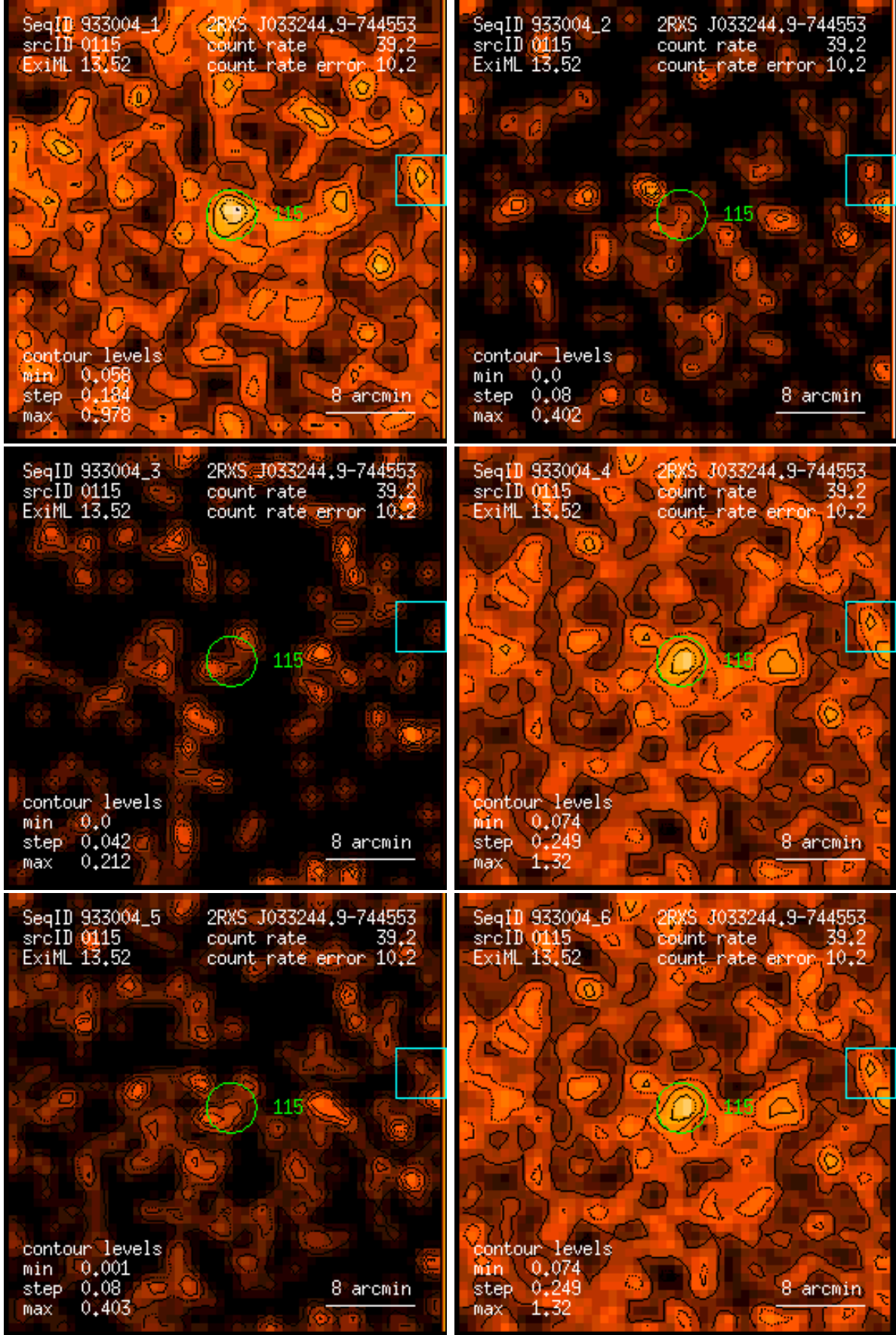
Figure 115: RASS 933004: detection 0115: band rate images, Gaussian filter: (1) PSPC channels 11 – 41, (2) 52 – 90, (3) 91 – 201, (4) 11 – 235, (5) 52 – 201, (6) 11 – 201. Broad band rates in counts/ks. Band rate contour levels in counts/ks/arcmin 2 .
