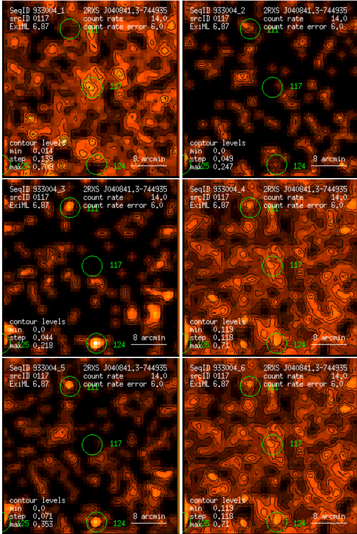
Figure 117: RASS 933004: detection 0117: band rate images, Gaussian filter: (1) PSPC channels 11 – 41, (2) 52 – 90, (3) 91 – 201, (4) 11 – 235, (5) 52 – 201, (6) 11 – 201. Broad band rates in counts/ks. Band rate contour levels in counts/ks/arcmin 2 .
