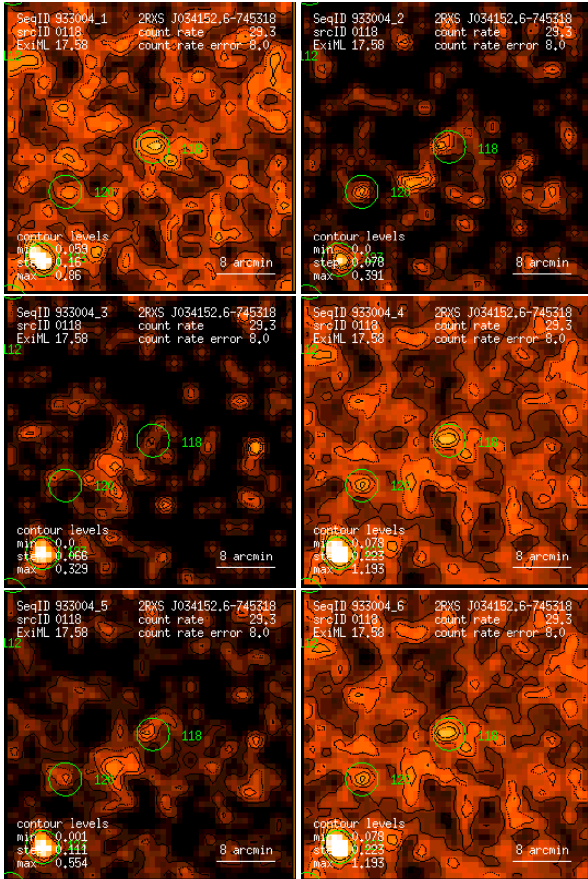
Figure 118: RASS 933004: detection 0118: band rate images, Gaussian filter: (1) PSPC channels 11 – 41, (2) 52 – 90, (3) 91 – 201, (4) 11 – 235, (5) 52 – 201, (6) 11 – 201. Broad band rates in counts/ks. Band rate contour levels in counts/ks/arcmin 2 .
