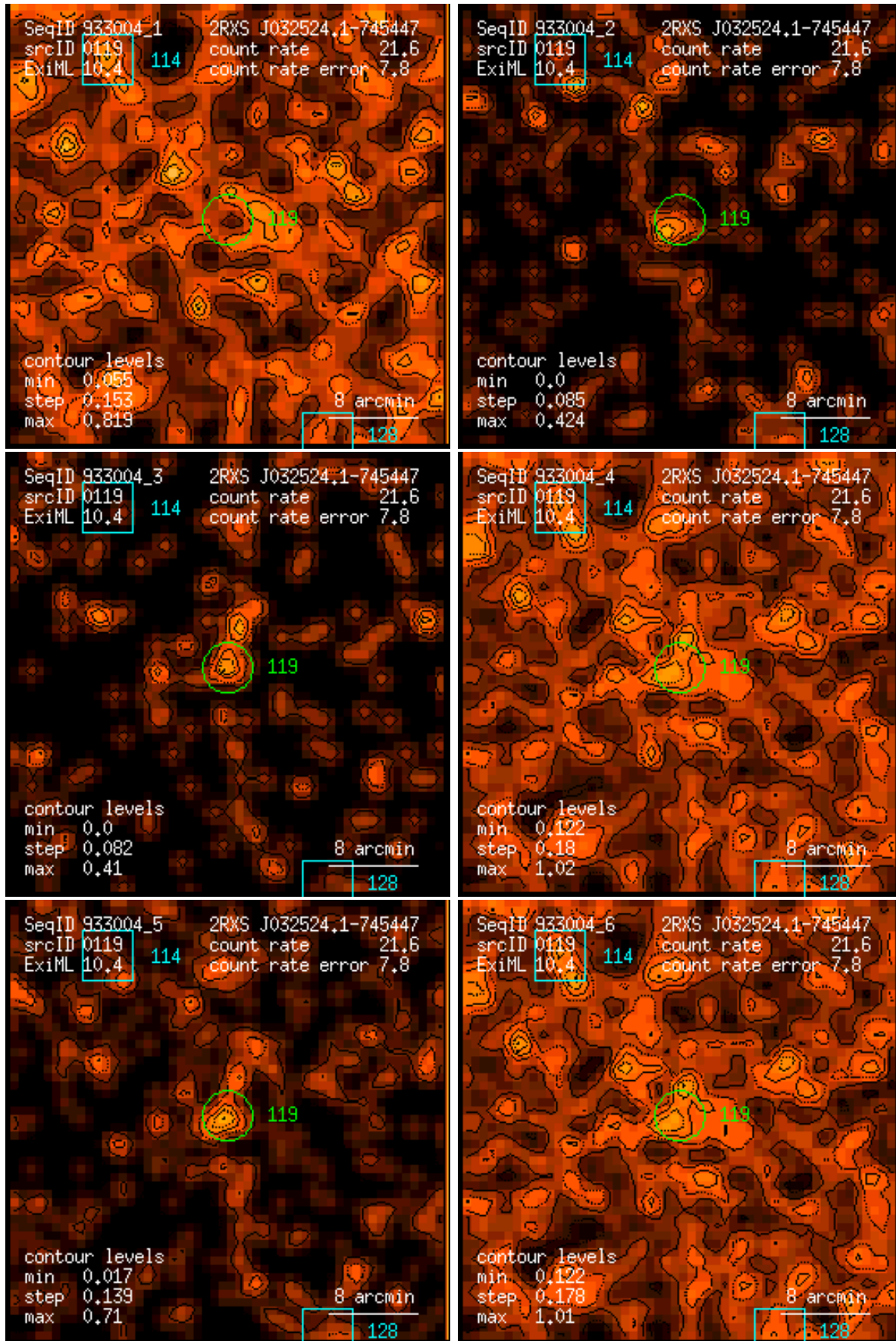
Figure 119: RASS 933004: detection 0119: band rate images, Gaussian filter: (1) PSPC channels 11 – 41, (2) 52 – 90, (3) 91 – 201, (4) 11 – 235, (5) 52 – 201, (6) 11 – 201. Broad band rates in counts/ks. Band rate contour levels in counts/ks/arcmin 2 .
