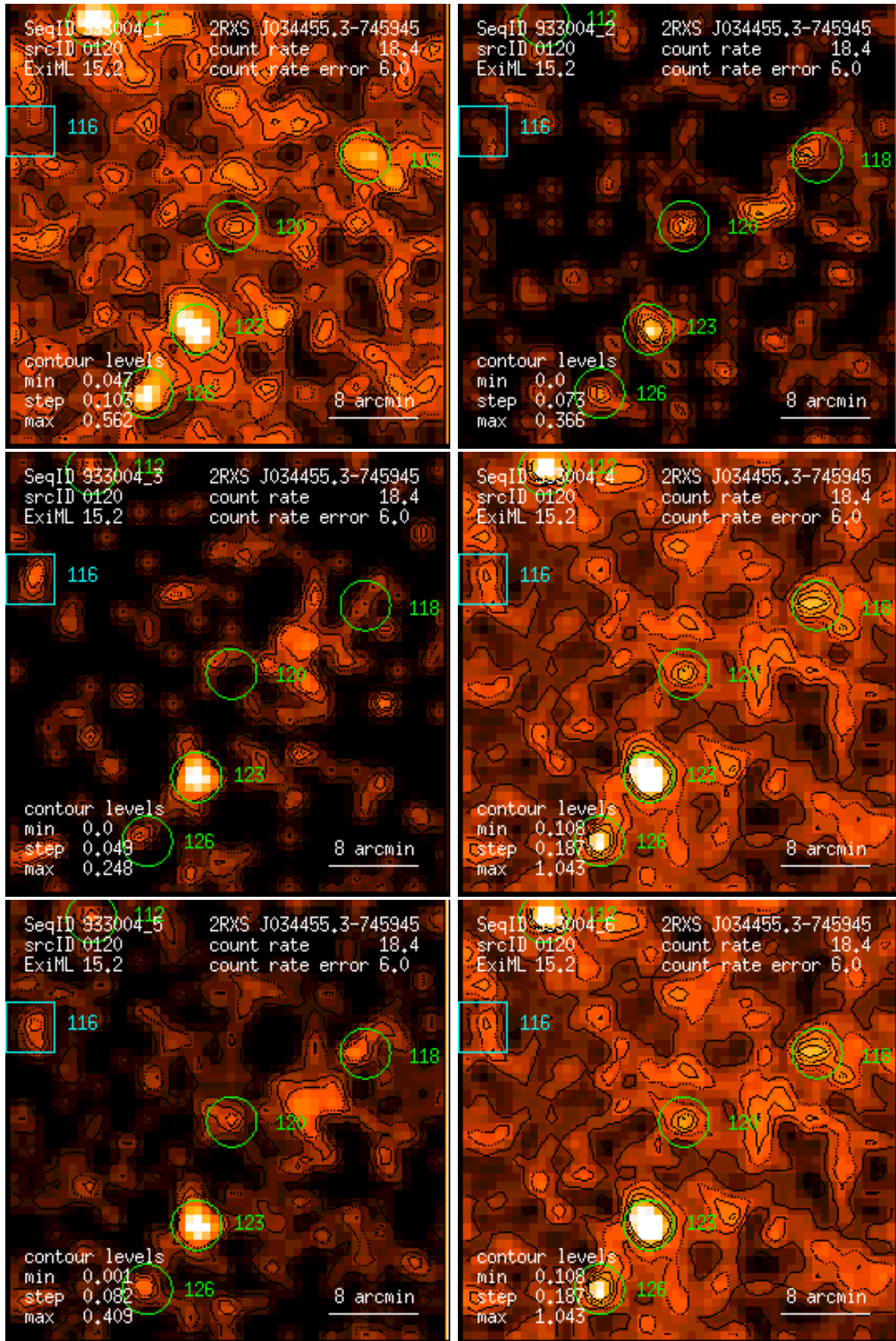
Figure 120: RASS 933004: detection 0120: band rate images, Gaussian filter: (1) PSPC channels 11 – 41, (2) 52 – 90, (3) 91 – 201, (4) 11 – 235, (5) 52 – 201, (6) 11 – 201. Broad band rates in counts/ks. Band rate contour levels in counts/ks/arcmin 2 .
