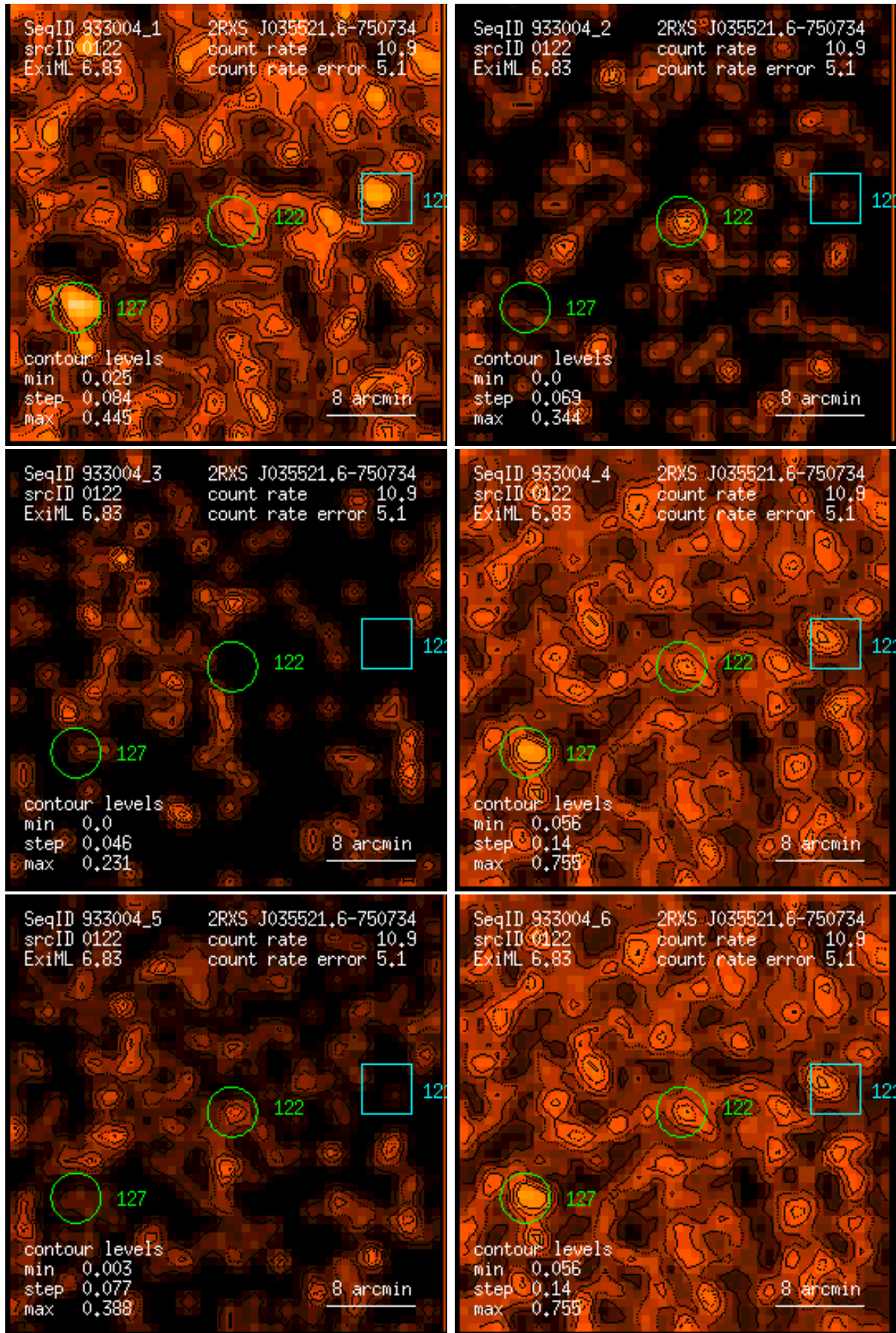
Figure 122: RASS 933004: detection 0122: band rate images, Gaussian filter: (1) PSPC channels 11 – 41, (2) 52 – 90, (3) 91 – 201, (4) 11 – 235, (5) 52 – 201, (6) 11 – 201. Broad band rates in counts/ks. Band rate contour levels in counts/ks/arcmin 2 .
