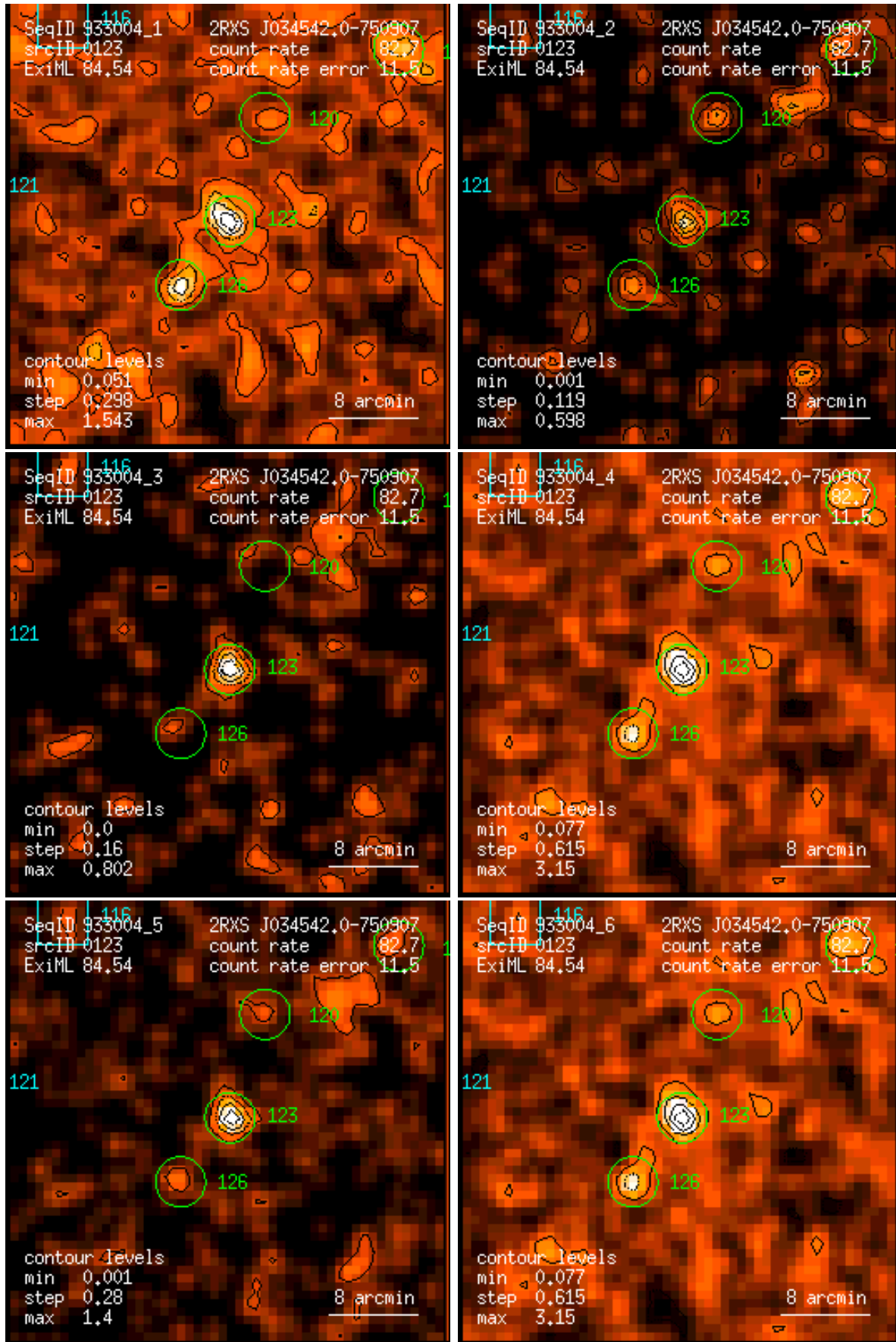
Figure 123: RASS 933004: detection 0123: band rate images, Gaussian filter: (1) PSPC channels 11 – 41, (2) 52 – 90, (3) 91 – 201, (4) 11 – 235, (5) 52 – 201, (6) 11 – 201. Broad band rates in counts/ks. Band rate contour levels in counts/ks/arcmin 2 .
