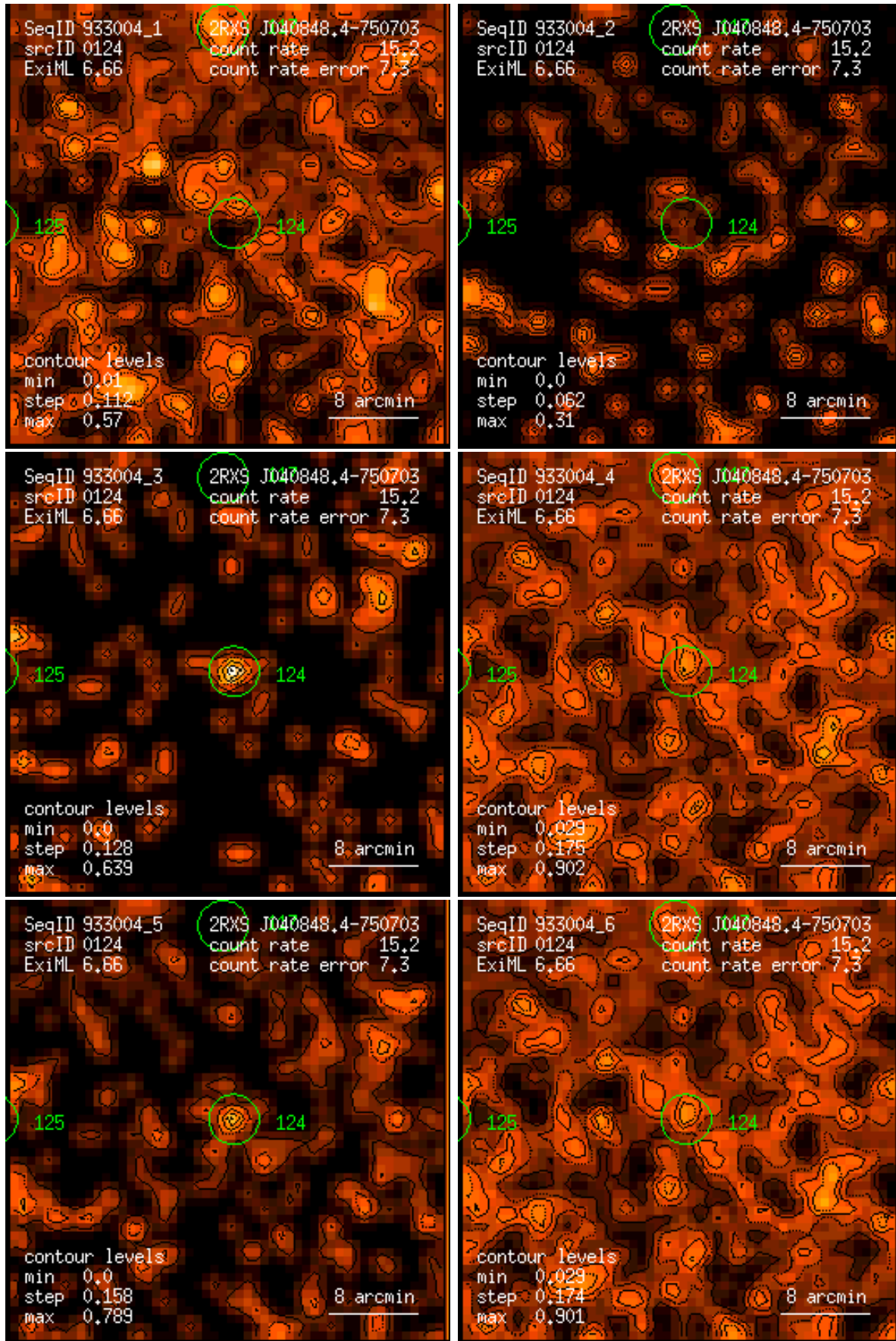
Figure 124: RASS 933004: detection 0124: band rate images, Gaussian filter: (1) PSPC channels 11 – 41, (2) 52 – 90, (3) 91 – 201, (4) 11 – 235, (5) 52 – 201, (6) 11 – 201. Broad band rates in counts/ks. Band rate contour levels in counts/ks/arcmin 2 .
