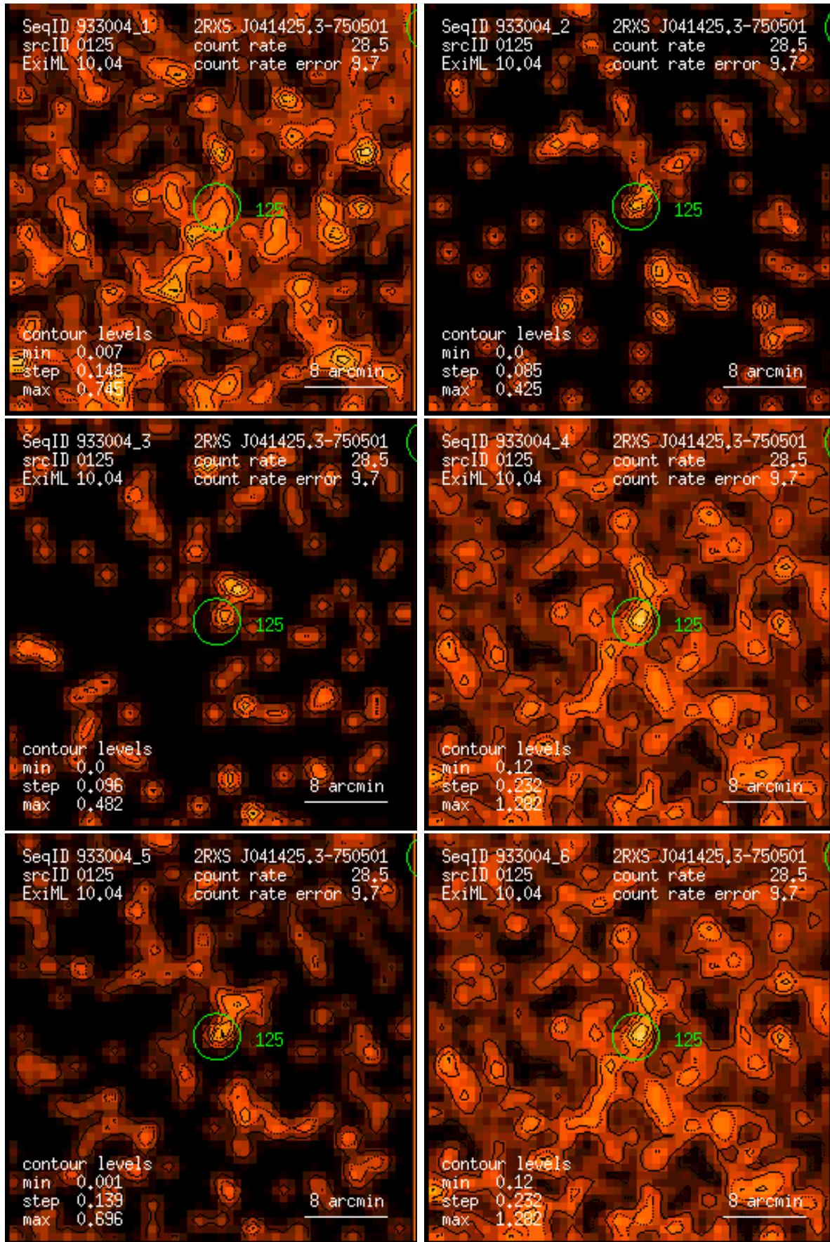
Figure 125: RASS 933004: detection 0125: band rate images, Gaussian filter: (1) PSPC channels 11 – 41, (2) 52 – 90, (3) 91 – 201, (4) 11 – 235, (5) 52 – 201, (6) 11 – 201. Broad band rates in counts/ks. Band rate contour levels in counts/ks/arcmin 2 .
