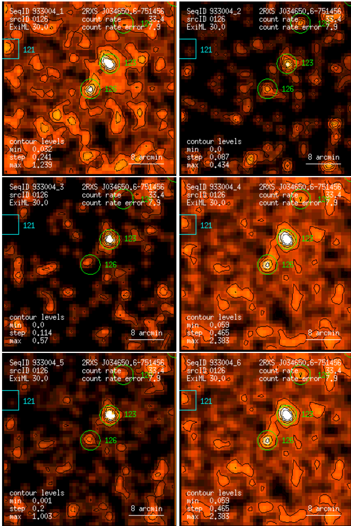
Figure 126: RASS 933004: detection 0126: band rate images, Gaussian filter: (1) PSPC channels 11 – 41, (2) 52 – 90, (3) 91 – 201, (4) 11 – 235, (5) 52 – 201, (6) 11 – 201. Broad band rates in counts/ks. Band rate contour levels in counts/ks/arcmin 2 .
