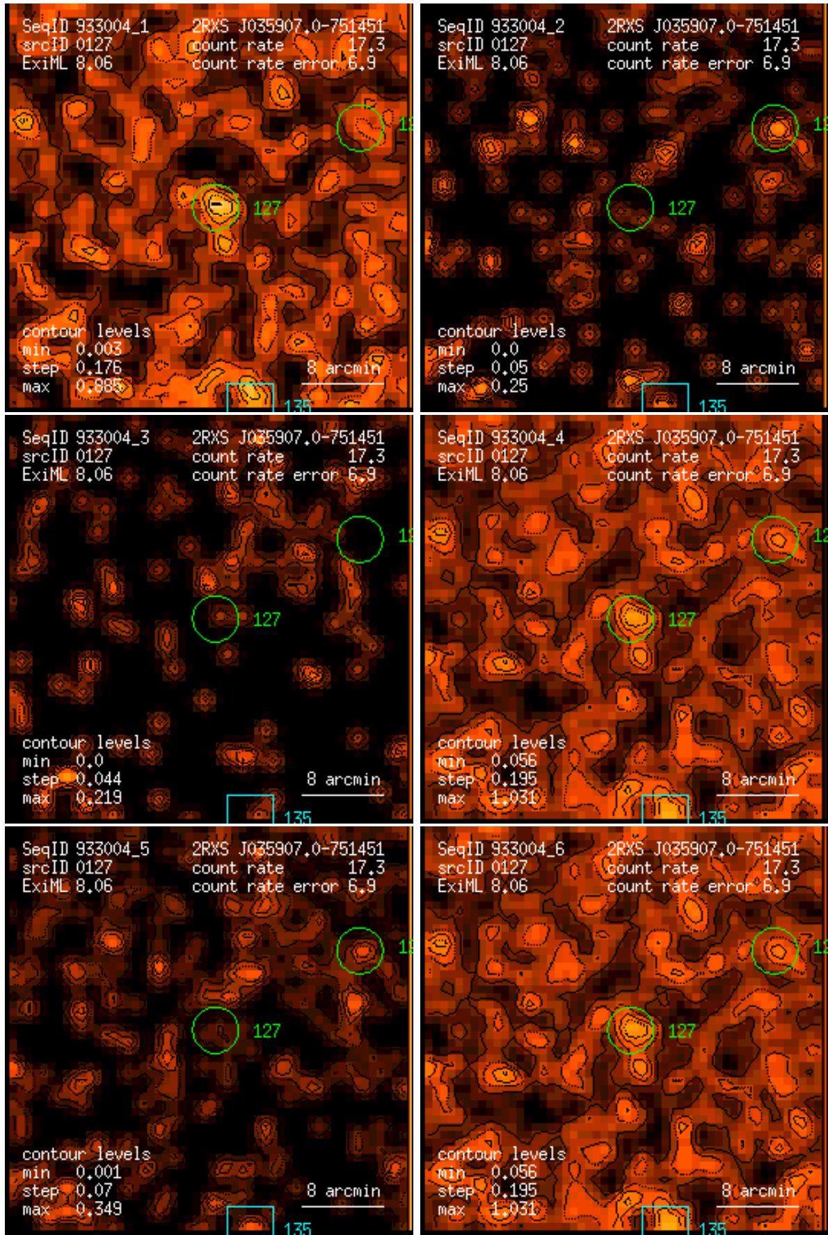
Figure 127: RASS 933004: detection 0127: band rate images, Gaussian filter: (1) PSPC channels 11 – 41, (2) 52 – 90, (3) 91 – 201, (4) 11 – 235, (5) 52 – 201, (6) 11 – 201. Broad band rates in counts/ks. Band rate contour levels in counts/ks/arcmin 2 .
